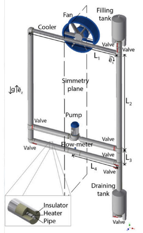
Figure 6. The DYNASTY facility at PoliMi.
