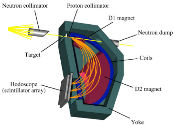
Fig. 2. magnetic MPR spectrometer with removed magnet yoke lid.
