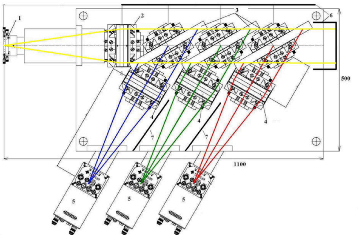
Figure 10. Principle scheme of the multi-channel HES spectrometer. 1 - entrance slit; 2 -collimator objective lens; 3 - holographic transmission gratings for 468 \pm 5 nm, 529 \pm 5 nm and 656 \pm 6 nm spectral ranges; 4 - camera objective lenses; 5 - CCD cameras; 6 - light traps/viewing dumps; 7 - light shields/baffles.
