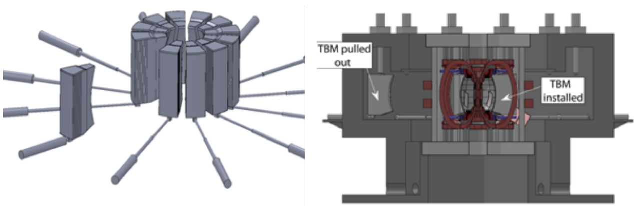
Fig. 4. Blanket maintenance approach, proposal for DEMO TBM tests
