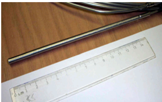
Fig. 2 : a) Picture of the prototype SPND with Cr emitter; b) Measured "dark" current of the SPND_Cr detector at 400 °C
