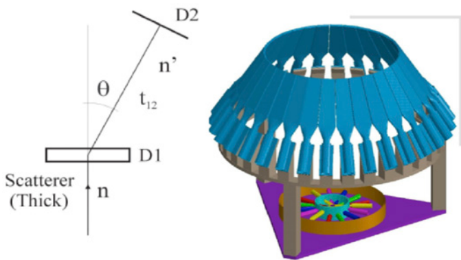
Fig. 1 The neutron TOF spectrometer principle and TOFOR design.
