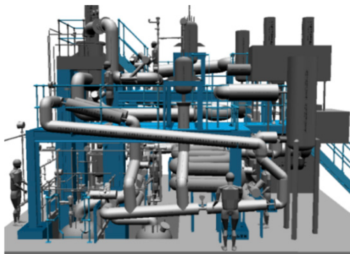
Fig.9. Dual Coolant Thermal Hydraulic Integrated Experimental Loop (DRAGON-V)
