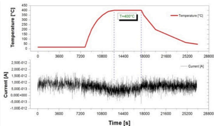
Fig. 2 : a) Picture of the prototype SPND with Cr emitter; b) Measured "dark" current of the SPND_Cr detector at 400 °C
