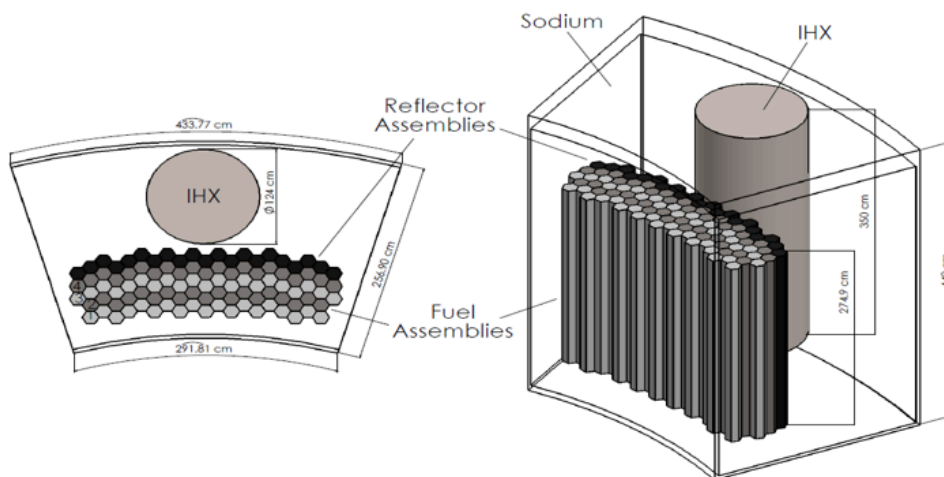
Fig. 2. SABR modular sodium pool with reactor and intermediate heat exchanger.
