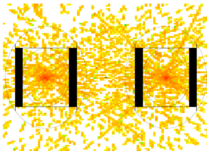
Fig. 4: Hybrid system horizontal (left) and vertical (right) sections in which it is possible to see the neutron source distribution.
