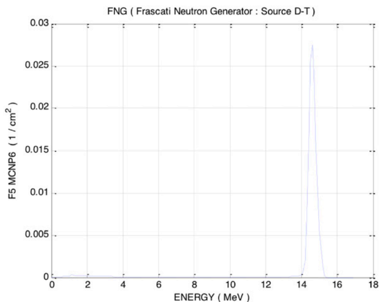
Figure 5: Neutron spectrum of FNG (Frascati Neutrons Generator) 14 MeV calculated at 0.5 cm from D-T source
