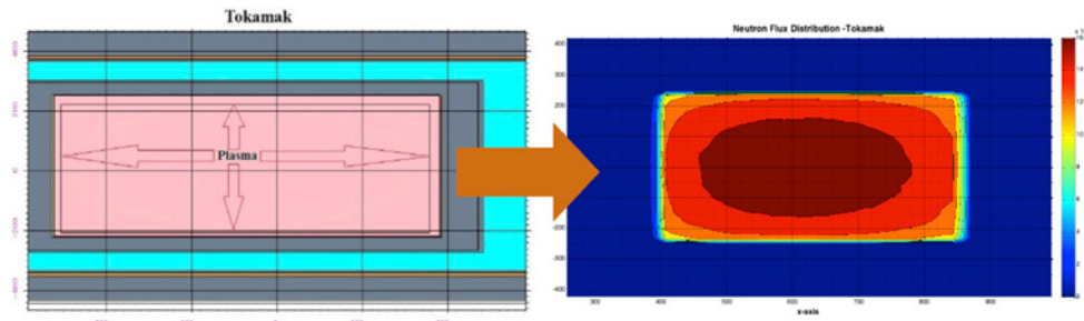
Figure 7. Axially NFP from the Tokamak by surfaces
