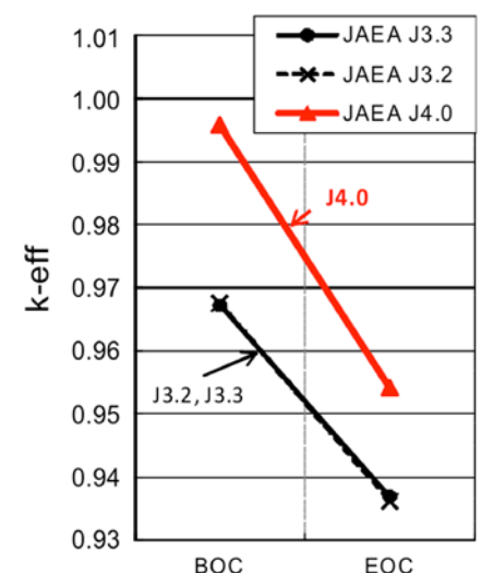
Fig. 7 Comparison of calculation results for k_{\text{eff}} with different version of JENDL libraries (BOC=beginning of cycle, EOC=end of cycle)
