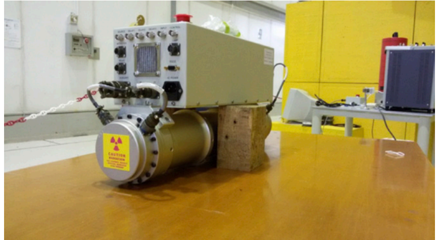
Figure 3: the portable neutron generator employed in the microexperiment performed at the ENEA Casaccia Center.
