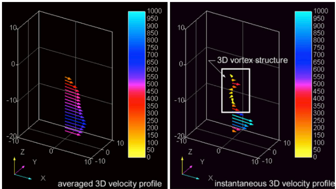
Fig.5 Averaged and instantaneous three-dimensional velocity vector profile in LBE loop measured by Vector-UVP system
