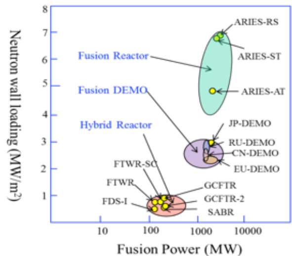
Fig.3. Neutron wall loading of a series of fusion and hybrid reactors
