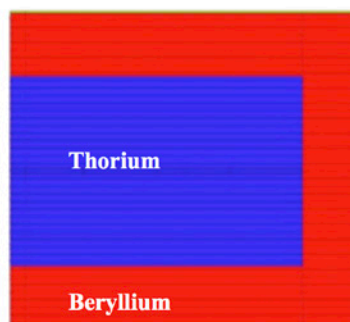
Fig.7 The geometry of MCNP model of the Thorium-Beryllium target : internal diameter is 60 cm, reflector's thickness is 20 cm, total length is 120 cm
