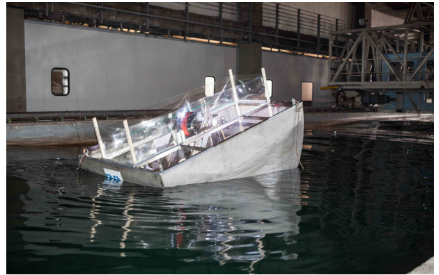
Figure 5 - The PEWEC prototype at INSEAN
