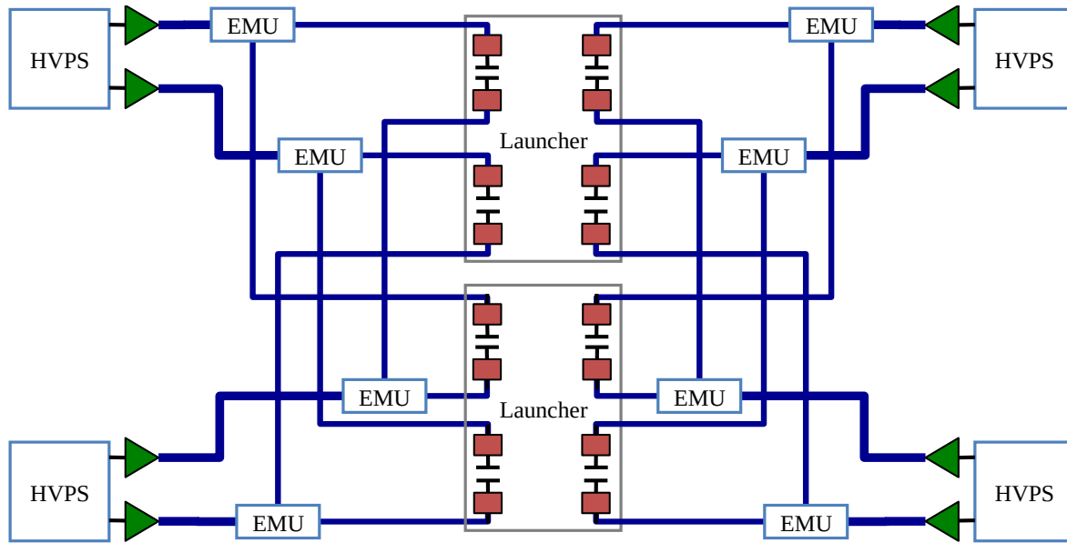
Figure 4.99: Feeding scheme of the straps of two launchers with eight external matching units (EMU).
