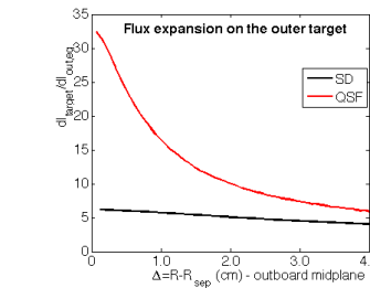
Figure 3.12: Flux expansion for SD (black) and QSF
