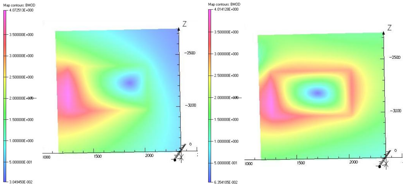
Figure 4.30: Magnetic field map for PF6 at t=0 s of RF(left) and for DN-SOF (left)
