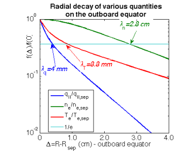
Figure 3.10: e-folding decay lengths
