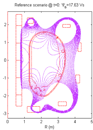
Figure 4.34: Reference SN scenario: pre-magnetization.
