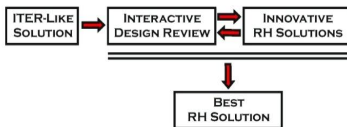
Figure 4.88: - Workflow scheme
