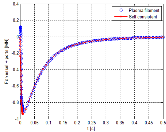
Figure 4.63: Assessment of force in the case of a purely filamentary current.
