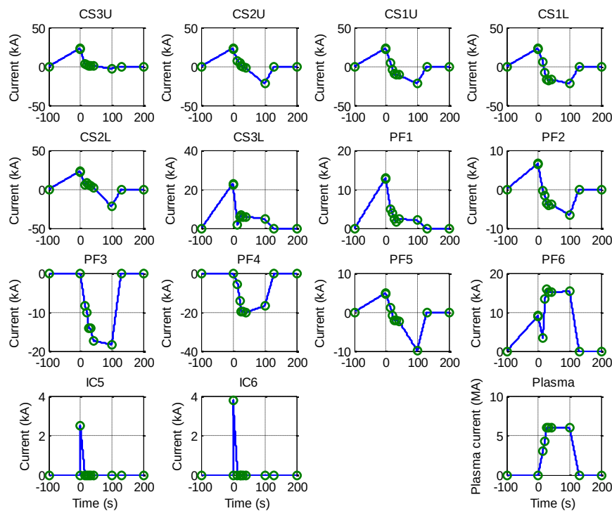
Figure 4.130: Current scenario for each magnetic coil.
