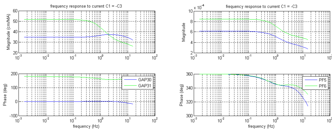
Figure 4.40: Use of in-vessel coils for strike point sweeping: dynamic response of the two strike points to a current flowing C1 and C3 connected in antiseres. The currents induced in PF5 and PF6 are also shown.
