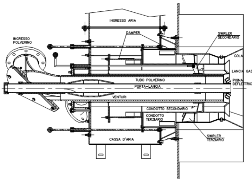
Figure 1. The burner section.
