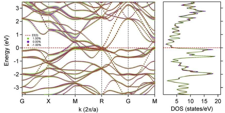
Fig. 2 The electronic band structure and density of states for Nb 3 Sn calculated for three representative strain states: +1.0 % (●), zero applied strain (◆), and -1.0 % (▲). The Fermi level is set to 0 eV.
