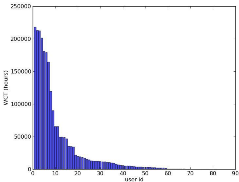
Fig. 2: WCT of CRESCO users in 2012 measured in hours vs. user id's.
