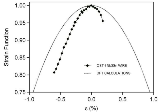
Fig.6 Direct comparison between the theoretical (dashed line) and experimental (line and markers) strain function [22]. The theoretical s(\varepsilon) correctly reproduces a bell shape, the mismatch being attributed to those extrinsic effects generally observed in technological wires.
