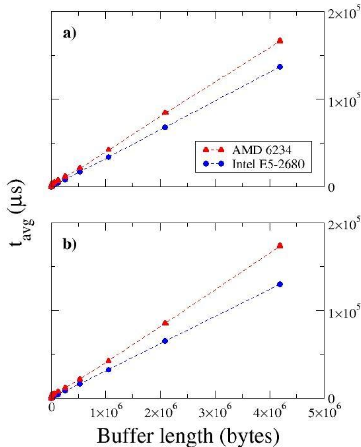
Figure 5: Intel MPI Alltoall benchmark. AMD 6234 vs. Intel E5-2680. a) Test compiled with GCC. b) Test compiled with Intel.
