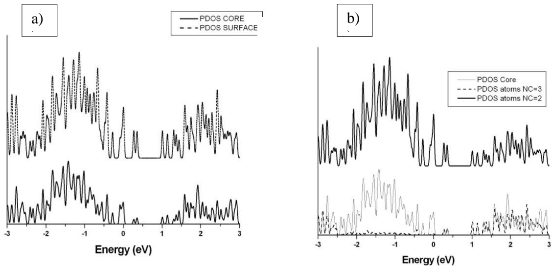
Figure 3: Partial density of states (PDOS) for CdS100; in figure 3a the contributions to the electronic states of the core atoms (solid line) and surface atoms (dashed line) have been reported. In figure 3b that of the surface contribution has been decomposed in two: dashed line for atoms with coordination NC = 3 and solid black line for atoms with coordination NC = 2.
