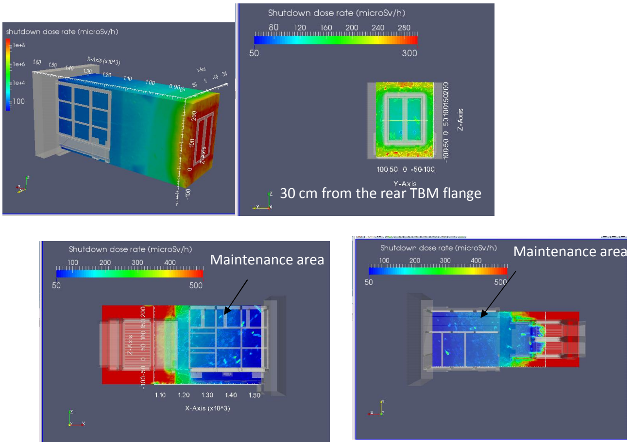
Fig. 3. Shutdown dose rate map at 12 days after shutdown in ITER equatorial TBM port. The dimension of the mesh element was 5 \times 5 \times 5 \text{ cm}^3 . Maps obtained running Advanced D1S on CRESCO_2 using 600 cores for 24h.
