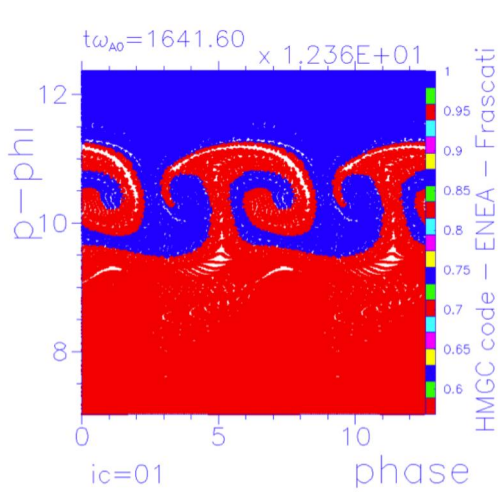
Fig. 3. Energetic particle orbits in the phase space coordinates (\Theta, P_\phi) .
