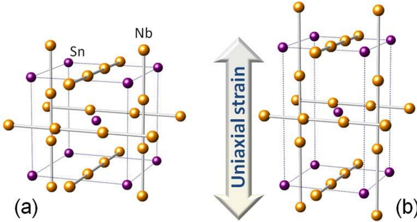
Fig. 1 The arrangement of atoms in the cubic (a) and tetragonal (b) phase of A15 Nb 3 Sn. The Nb atoms in the 2e sites form chains along the [001] direction, whereas those in the 4k sites are in chains along the [100] and [010] directions. To make the distortion clear, in (b), the cell is stretched to the abnormal value of \varepsilon = 40\% , whereas the Poisson's ratio \nu is set to 0.4.
