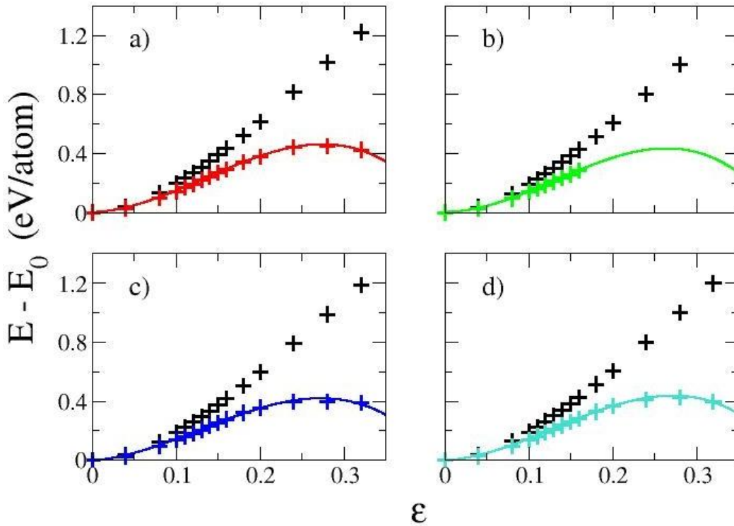
Figure 2: Total energy E per atom as a function of strain \epsilon for uniaxial deformation. a) bcc W monovacancy case; b) bcc W divacancy 1NN case; c) and d) bcc W divacancy 2NN case. For a), b) and c) uniaxial deformation in [001] direction. For d) uniaxial deformation in [100] direction. E_0 is the ground-state energy of the systems. Energies for unrelaxed conditions are shown in black symbols, those for relaxed conditions are shown in red, green, blue, and light blue symbols respectively. Solid lines are cubic fitting functions.
