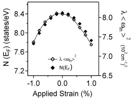
Fig.5 Density of states at Fermi level, N(E_F) , calculated as a function of strain. The curve is overlapped to the product function \lambda \cdot \omega_n^2 , which in good approximation should be proportional to N(E_F) [21].
