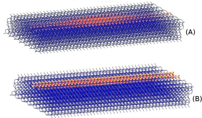
Figure 4: excitonic wavefunction of Si(111)2x1 positive buckling (A) and negative buckling (B).
