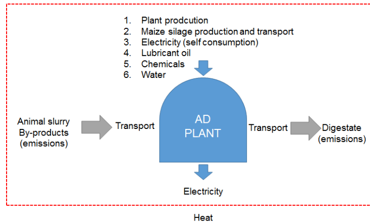
Figure 1: System boundary
