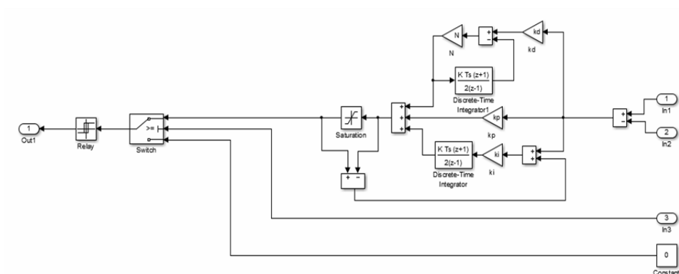
Figure 4.7: PID PWM digital controller block diagram.
