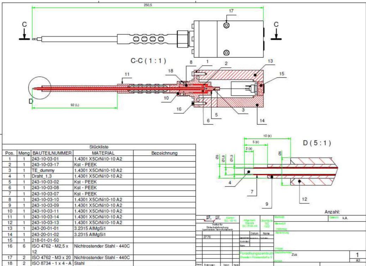
Figure 26. Conductivity sensors scheme
