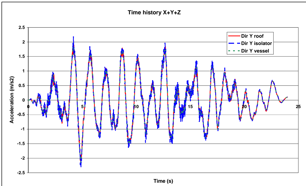
Figure 8 – Horizontal acceleration Y
