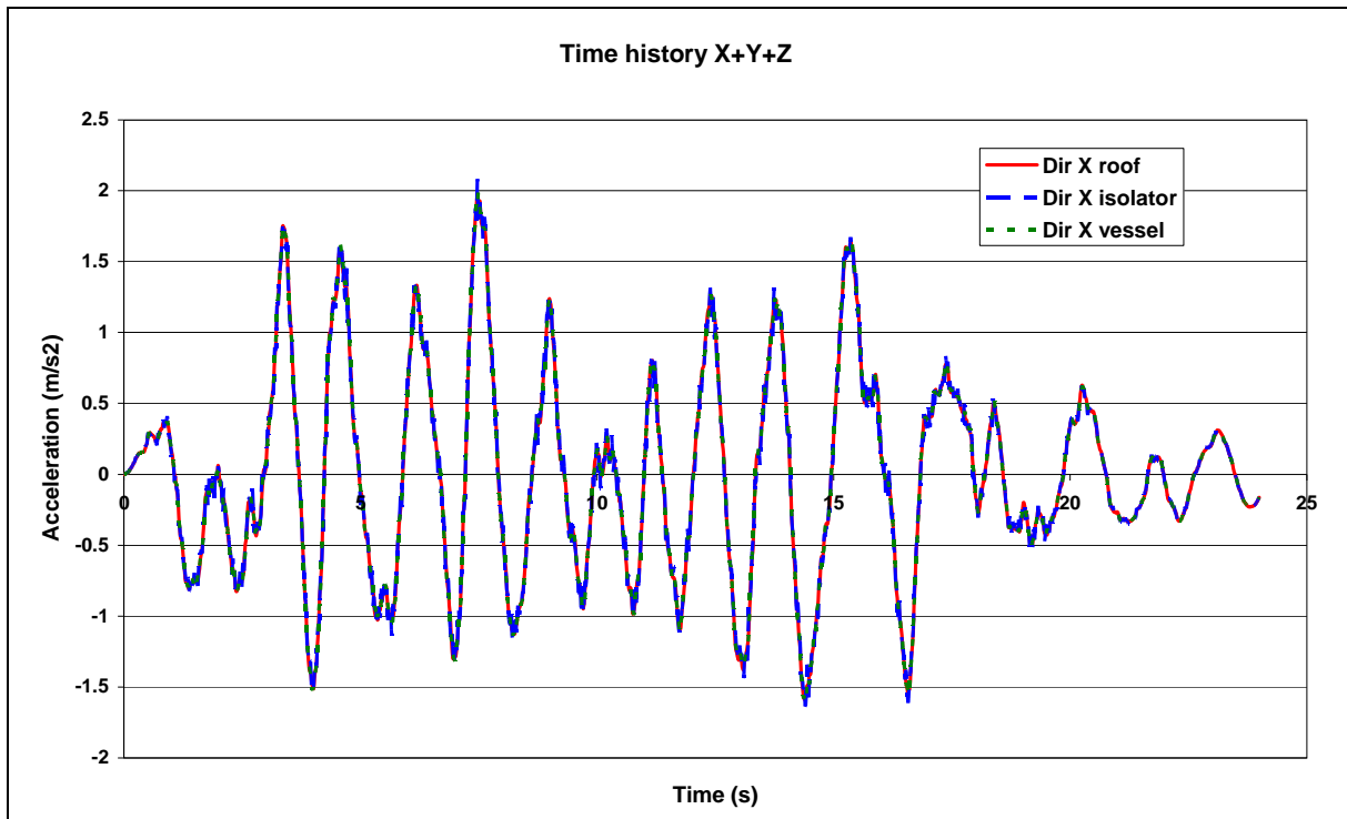
Figure 7 – Horizontal acceleration X
