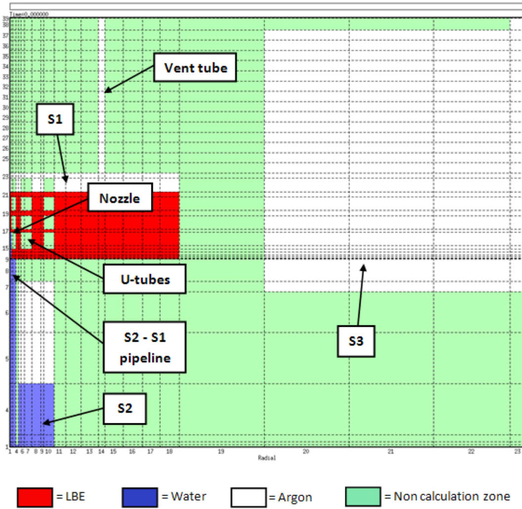
Figure 12 Two-dimensional model of LIFUS 5 used by SIMMER III code
