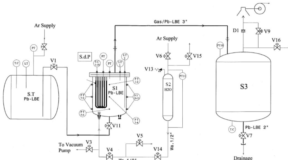
Figure 4 New LIFUS 5 layout
