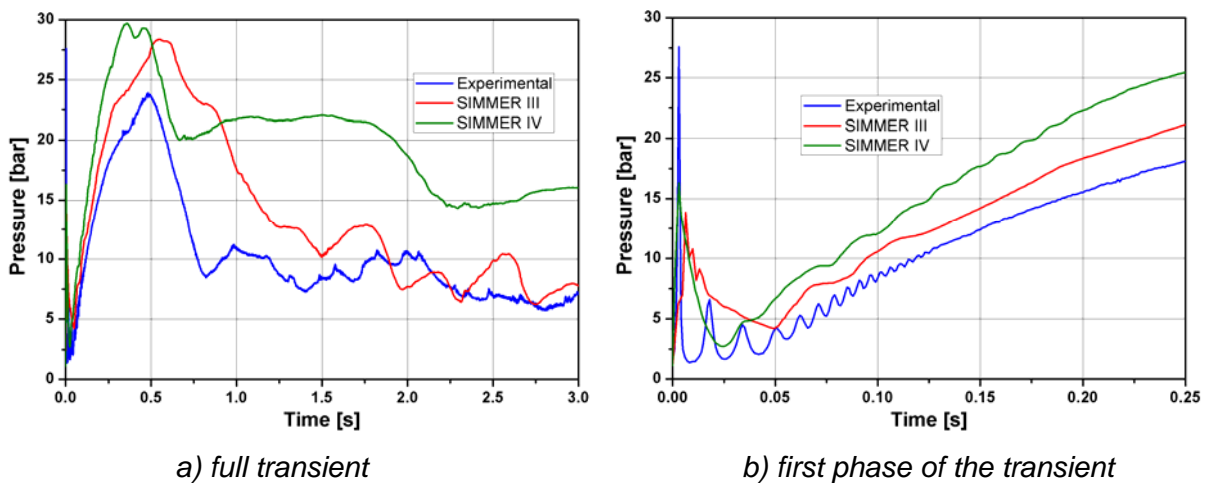
Figure 18 Pressure time trends for simulated and experimental data in PT7 location
