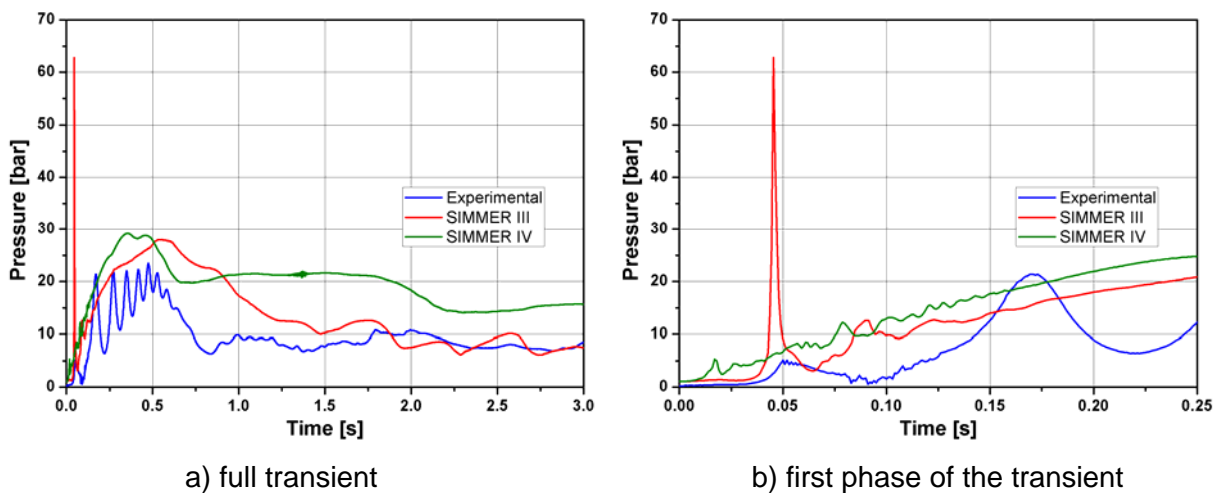
Figure 19 Pressure time trends for simulated and experimental data in PT3 location
