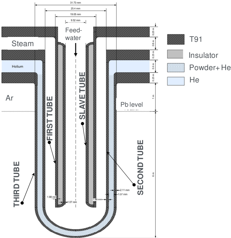
Fig. 4 – ALFRED SG Bayonet Tube scheme.
