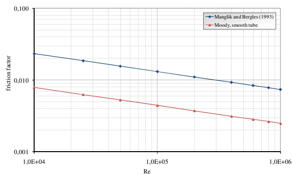
Fig. 72 – Twisted tapes insert, enhancement of the friction factor.
