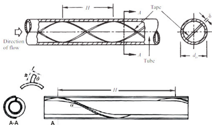
Fig. 70 – Scheme of twisted tape in circular tube and in a annular space.
