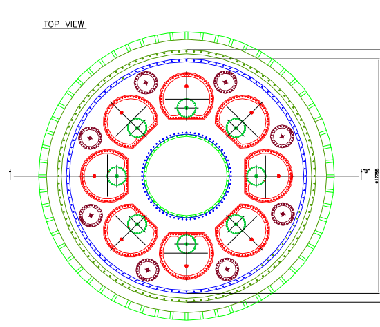
Fig. 2 – ALFRED primary system configuration.
