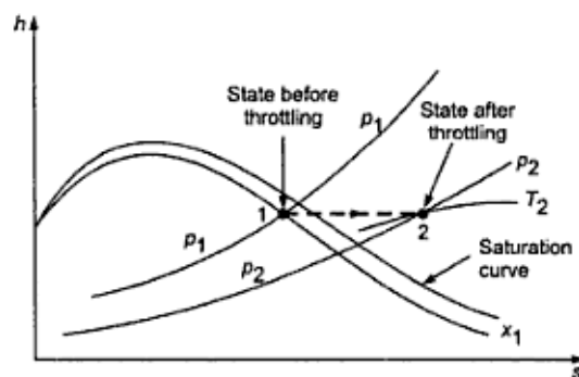
Fig. 82 – Throttling calorimeter: thermodynamic process h - S diagram.
