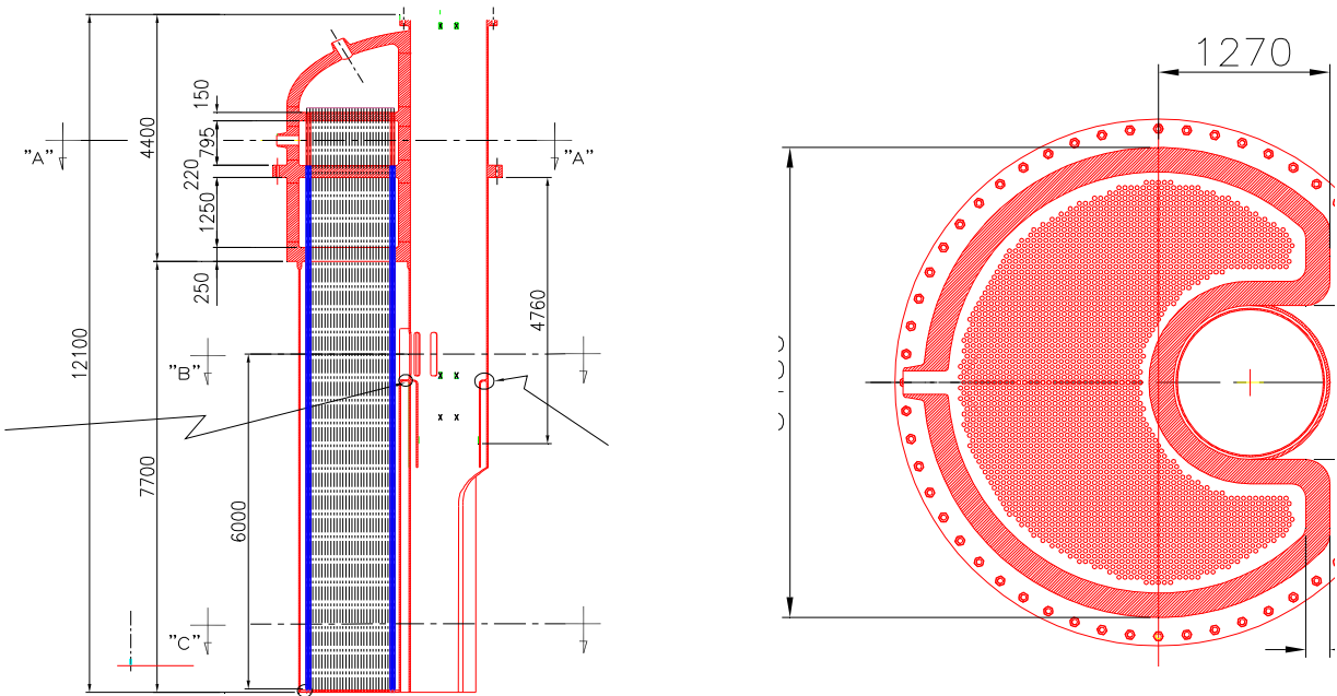
Fig. 3 – ALFRED SG conceptual design.
