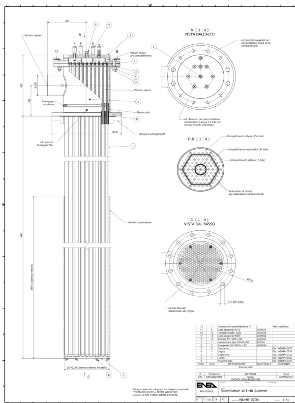
Fig. 1 – Double wall once through bayonet Heat Exchanger of CIRCE.
