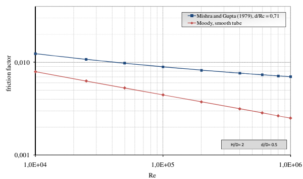
Fig. 77 – Coiled tube, enhancement of the friction factor.
