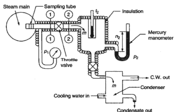
Fig. 81 – Throttling calorimeter scheme.
