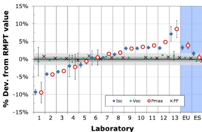
FIGURE 4 Percentage deviations from ESTI RMPT value for I_{\text{SC}} , V_{\text{OC}} , P_{\max} and FF of RR82 ( \mu\text{c-Si} ). RMPT value is represented by the x-axis, and its combined expanded UC ( k = 2 ) is shown for simplicity only for P_{\max} (light-grey-shaded area) and FF (dark-grey-shaded area). The error bars shown represent the UC of the submitted result as stated by the participant. The EU and ES values correspond to the ESTI measurements made, respectively, before and after the pre-conditioning at the end of the RR PT. Note that the laboratory identification number may be different for the other DUTs [Colour figure can be viewed at wileyonlinelibrary.com ]
