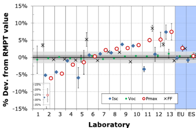
FIGURE 7 Percentage deviations from ESTI RMPT value for I_{SC} , V_{OC} , P_{\max} and FF of RR85 (a-Si/ \mu c-Si). RMPT value is represented by the x-axis and its combined expanded UC ( k = 2 ) is shown for simplicity only for P_{\max} (light-grey-shaded area) and FF (dark-grey-shaded area). The error bars shown represent the UC of the submitted result as stated by the participant. An inset is shown for the points falling outside the main range of the deviations. The EU and ES values correspond to the ESTI measurements made, respectively, before and after the pre-conditioning at the end of the RR PT. Note that the laboratory identification number may be different for the other DUTs [Colour figure can be viewed at wileyonlinelibrary.com ]
