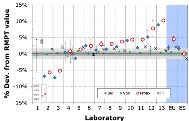
FIGURE 5 Percentage deviations from ESTI RMPT value for I_{\text{SC}} , V_{\text{OC}} , P_{\max} and FF of RR83 (a-Si/ \mu\text{c-Si} ). RMPT value is represented by the x-axis, and its combined expanded UC ( k = 2 ) is shown for simplicity only for P_{\max} (light-grey-shaded area) and FF (dark-grey-shaded area). The error bars shown represent the UC of the submitted result as stated by the participant. The EU and ES values correspond to the ESTI measurements made, respectively, before and after the pre-conditioning at the end of the RR PT. An inset is shown for the points falling outside the main range of the deviations. Note that the laboratory identification number may be different for the other DUTs [Colour figure can be viewed at wileyonlinelibrary.com ]
