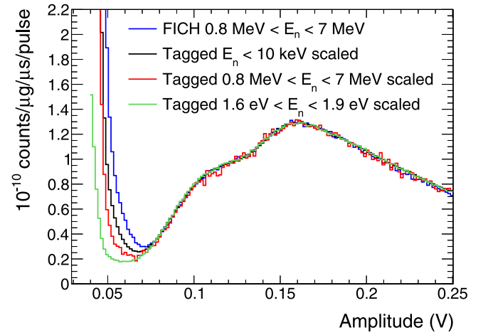
Fig. 17. Pulse height spectra of the events in the fission chamber for 0.8\text{ MeV} < E_n < 7\text{ MeV} compared to tagged events for different E_n regions from all FICH channels. The neutron flux of n_{TOF} can be seen in Fig. 7.
