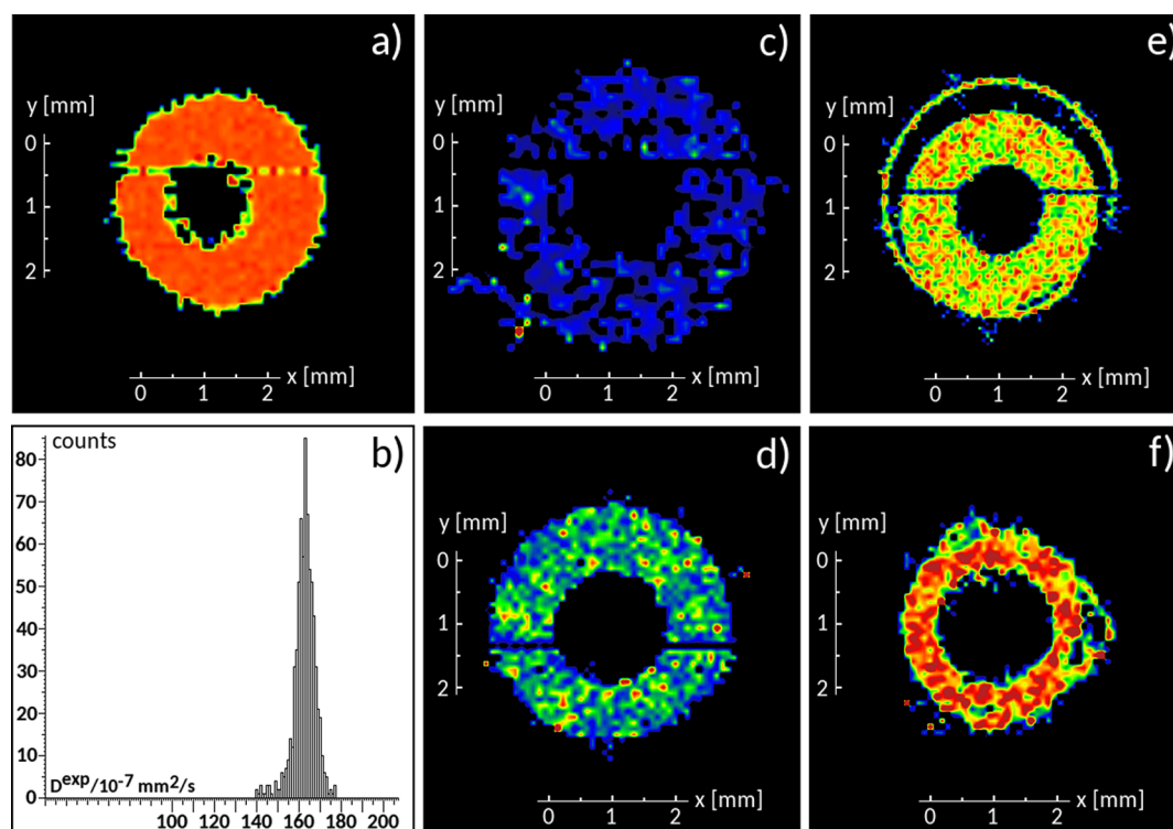
Figure 3. (a) DW image of neat PYR 14 TFSI at 19 °C; (b) corresponding diffusivity histogram. DW images at 19 °C for the samples (c) SPE2, (d) SPE3, (e) SPE4, and (f) SPE5. For better clarity, the diffusion coefficients are color-coded as follows: (a) 256 gradations from blue ( D = 1 \times 10^{-6} \text{ mm}^2/\text{s} ) to red ( D = 200 \times 10^{-6} \text{ mm}^2/\text{s} ); (c–f): 256 color gradations from blue ( D = 0.1 \times 10^{-6} \text{ mm}^2/\text{s} ) to red ( D = 15 \times 10^{-6} \text{ mm}^2/\text{s} ). In all DW images, the xy resolution is 63 \times 63 \mu\text{m}^2/\text{pixel} .
