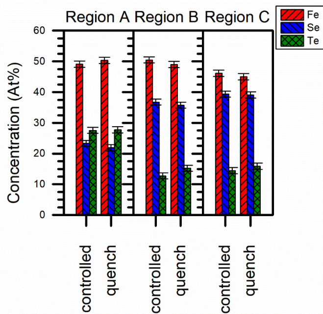
Figure 4. Summary of the results of EDS analyses carried out on the different samples regions (see text for details).
