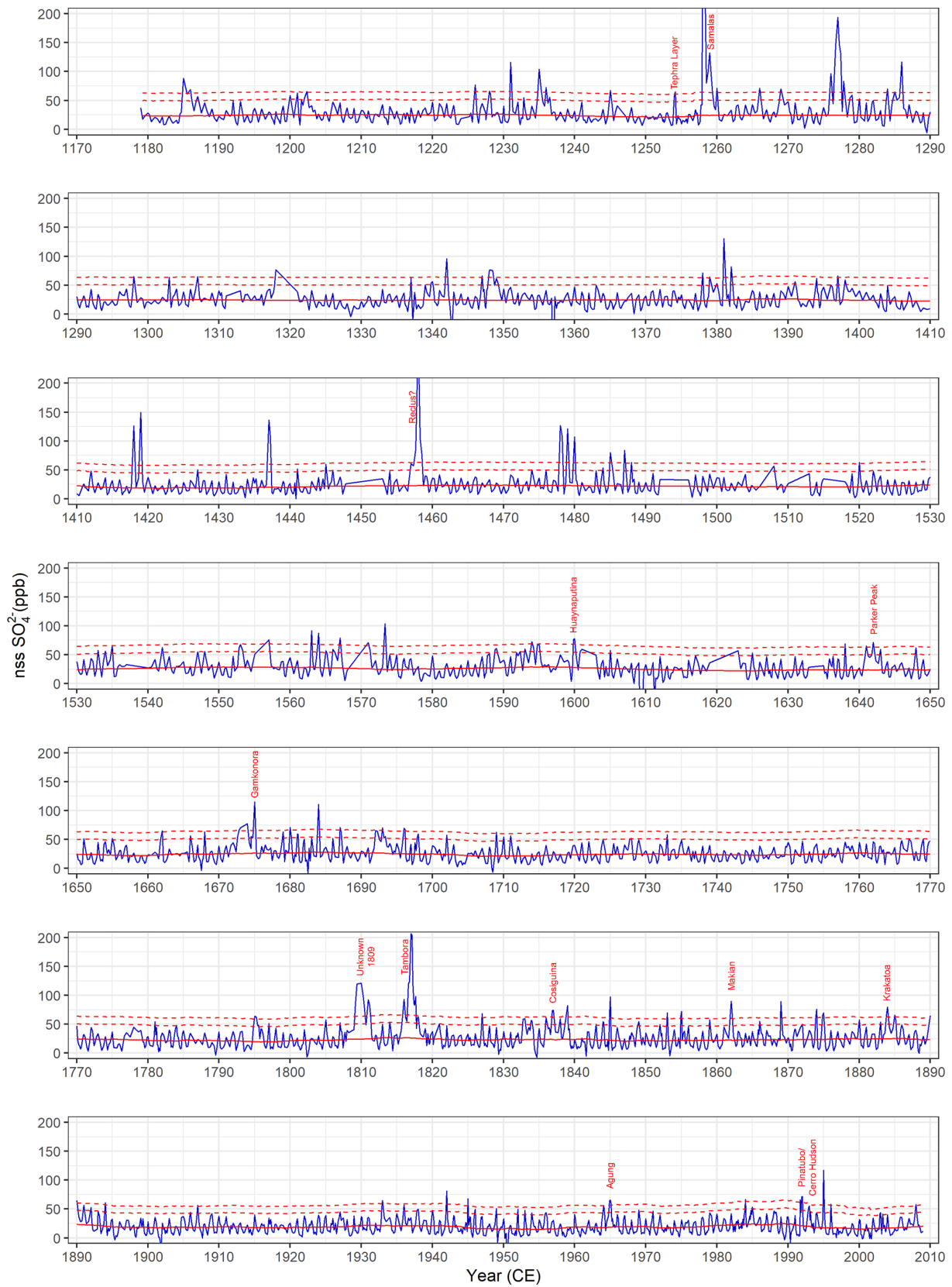
Figure 4. GV7(B) nssSO 4 2- profile plotted on the age scale produced in this paper. Biogenic background (solid red) and thresholds used to identify the volcanic signatures (2σ and 3σ, dashed red) are also reported.
