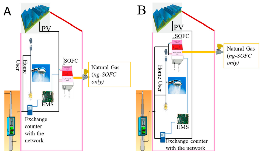
Figure 1. (A) Configuration with the fuel cells in front of the meter (i–iii). (B) Configuration installing the fuel cell behind the meter (ii–iv).
