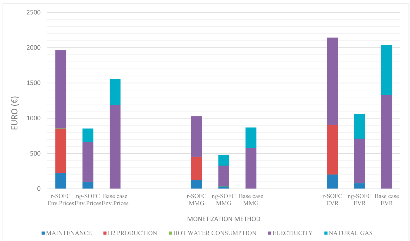
Figure 7. Total environmental costs for each method.
