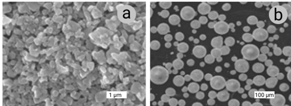
Figure 5. Morphology of powders: (a) Al 2 O 3 submicron powders, mean particle size 0.7 μm, prod. Alcoa A16SG, specific surface area 8.9 m 2 /g, shape factor β = 1.42; (b) ZrO 2 granules TZ-3Y, partially stabilized zirconia powder with a uniform dispersion of 3 mol % yttria, 40 nm, prod. Tosoh Corporation.
