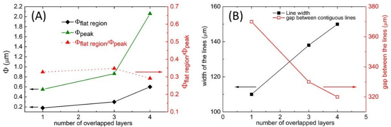
Figure 3. Geometric parameters measured for the PVA lines deposited on PLA substrate (see optical images, displayed in Figure 2). (A) Thickness ( \Phi ) of the flat region and lateral peaks of the printed line and their ratio. (B) Line width and gap between consecutive lines. The arrays are obtained by changing only the number of overlapped printed layers.
