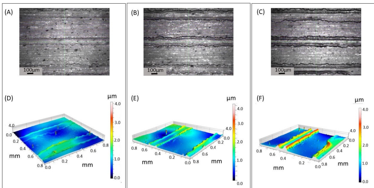
Figure 2. Optical microscopies (A–C) and optical profiles (D–F) of the PVA surface arrays printed onto PLA substrates, obtained by fixing the drop space and the nozzle number ( DS = 15 \mu\text{m} ; 4 nozzles) and by changing the number of overlapped layers: 1 layer (A,D), 3 layers (B,E), 4 layers (C,F).
