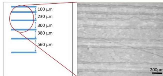
Figure 4. Scheme of deposited PVA pattern (left) and optical microscopy image (right) of an array of PVA lines printed onto PLA substrate, obtained by fixing the drop space ( DS = 15 \mu\text{m} ) and the overlapped layer number (2) as well as changing the gap between consecutive lines. The measured line width and thickness are 190 nm and 290 nm, respectively.
