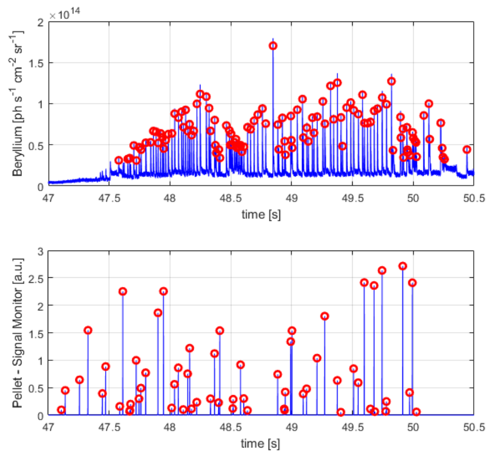
Figure 6. Pulse 92238. ELM signals with detected ELMs ( top ) and pellet monitor signals with detected Pellets ( bottom ) using the peak detection algorithm.
