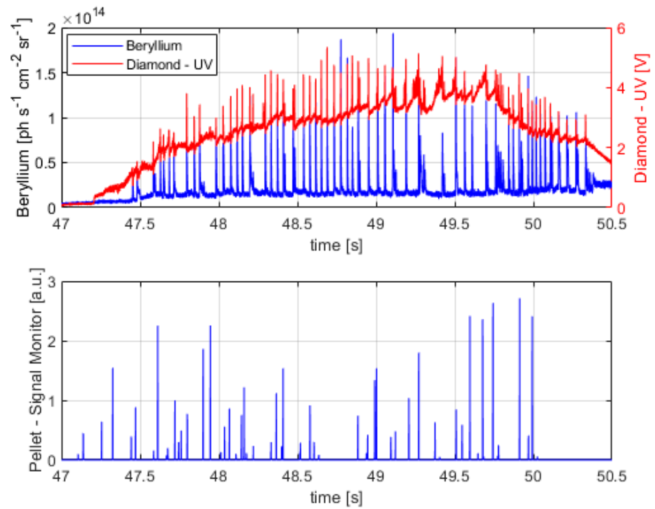
Figure 8. The ELM signals of shot 92237 ( top plot, beryllium in blue and diamond UV in red) and the pellet signal of shot 92238 ( bottom plot) used for the specificity analysis.
