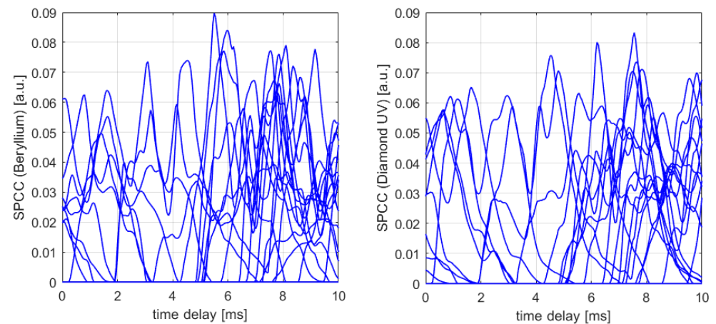
Figure 9. SPCC profiles ( left using beryllium line, right using diamond UV) of the detected ELMs of shot 92237 correlated with the pellet of shot 92238.
