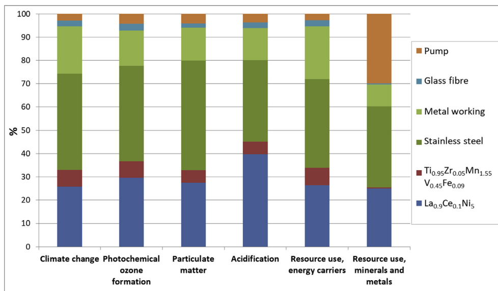
Fig. 3 – LCIA results, express as a percentage of the total, to produce of the MH compressor.
