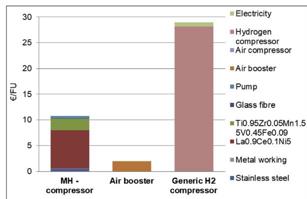
Fig. 7 – Cost for the compression of 1.79 kg of H_2 , at 200 bar, with the three systems analyzed. Because waste heat was considered to be supplied to the MH compressor, no energy costs were considered in the case. The use of energy from the Italian national mix was assumed to power the system with booster and the generic compressor for H_2 .
