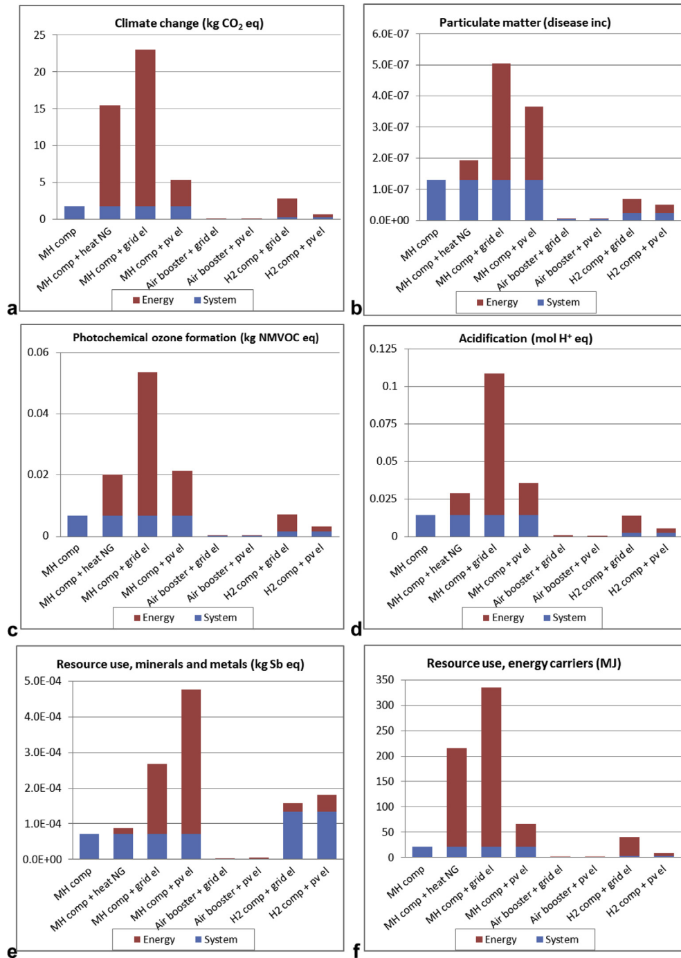
Fig. 5 – Comparison of the environmental impacts associated with the compression of 1.79 kg of H 2 at 200 bar using different systems. Impact categories: a) climate change, b) particulate matter, c) photochemical ozone formation, d) acidification, e) resource use, minerals and metals, f) resource use, energy carriers.
