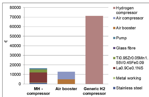
Fig. 6 – Capital cost of analyzed hydrogen compression systems.
