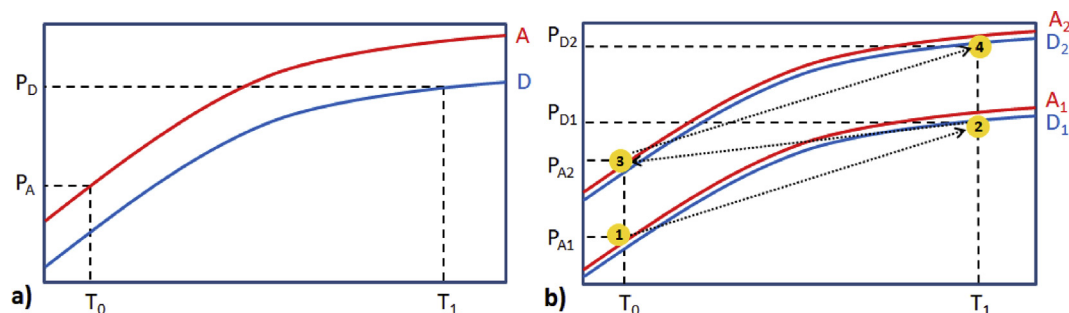
Fig. 1 – Pressure (P) - temperature (T) diagrams for the H_2 compression with metal hydride: a) absorption (A) and desorption (D) curves of a single solid phase; b) absorption and desorption curves of a system made of two connected solid phases.
