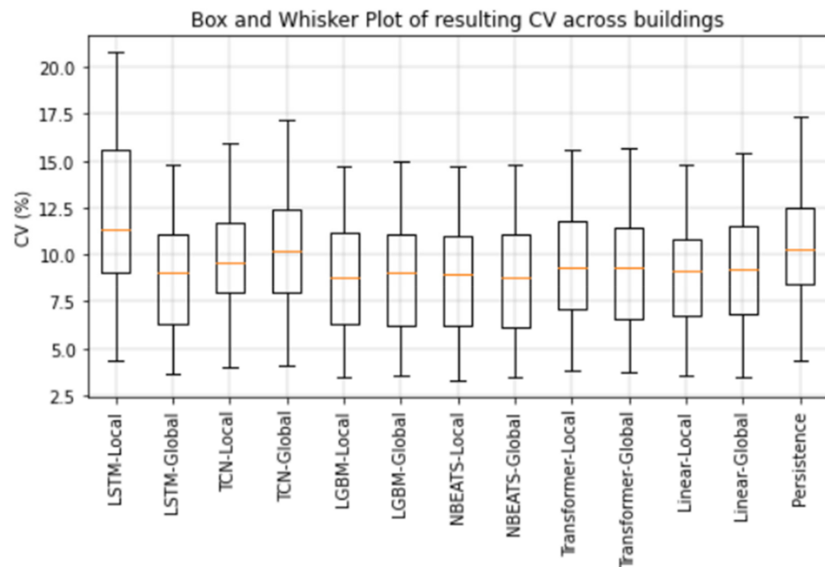
Figure 16. Comparison between the CV obtained from the considered local and global models on test set. The Persistence model has been added as a baseline.
