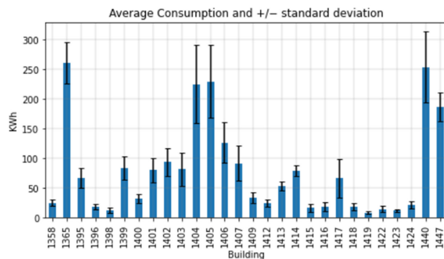
Figure 2. Hourly electricity consumption for the 28 considered buildings.
