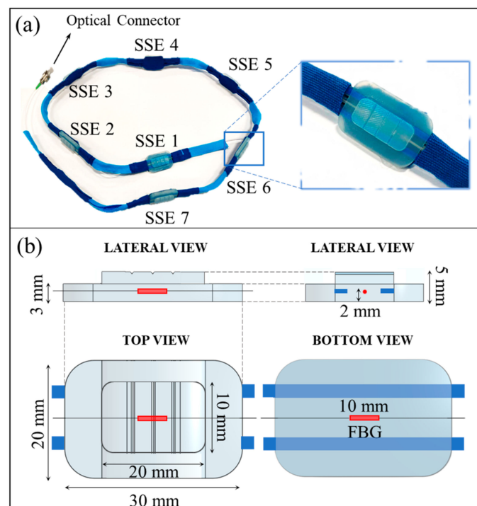
Figure 1. The wearable system. (a) A picture of the wearable system (on the left), together with a close-up view of one of the seven identical sensing elements (on the right); (b) Rendering and features of the sensing elements shown in lateral, top, and bottom views.
