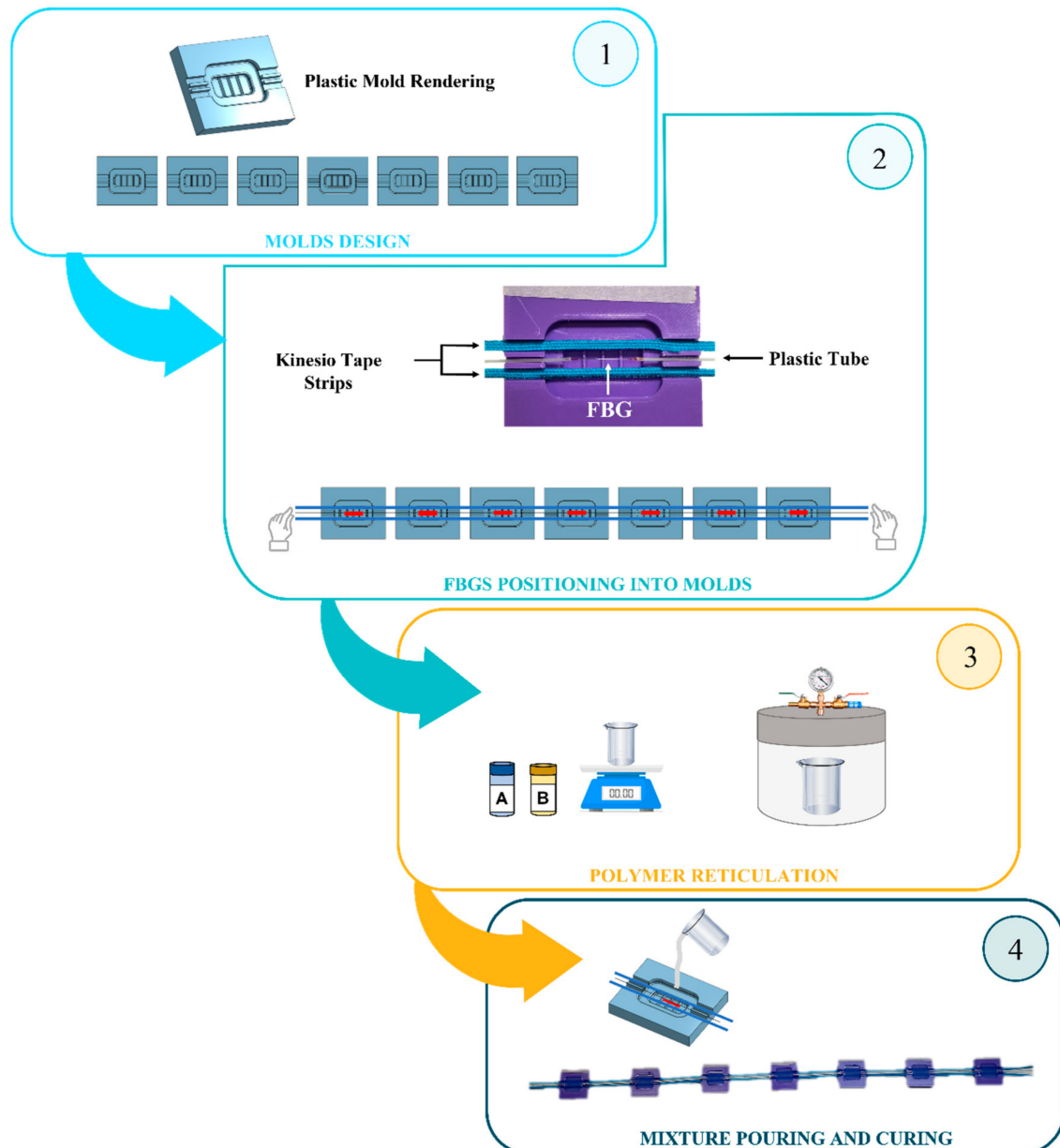
Figure 2. Diagram showing the manufacturing process of wearable system.
