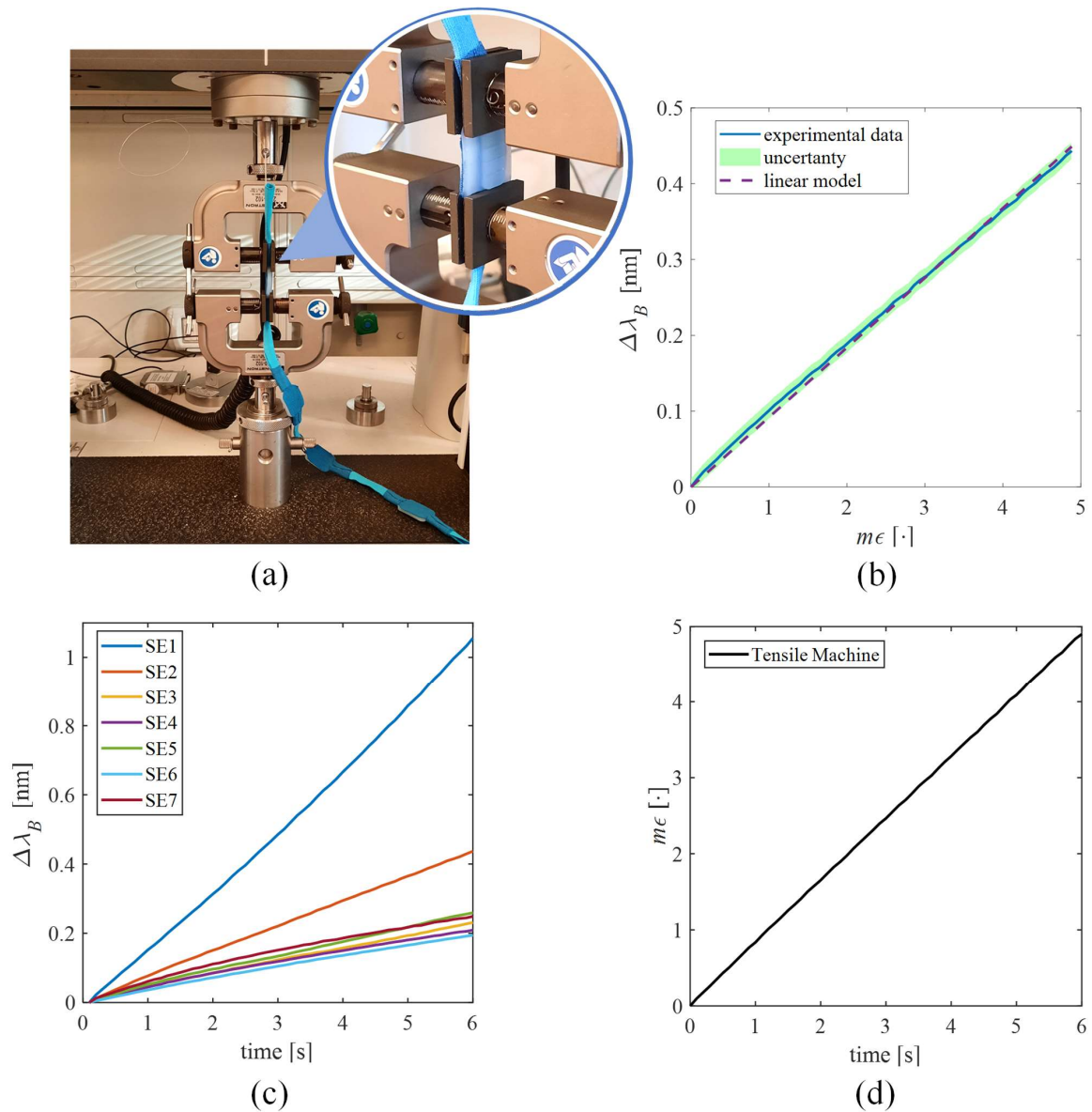
Figure 3. Response to strain of the SSEs. (a) The testing machine and a zoom of the sensing element placed between the two clamps. (b) The calibration curve of \Delta\lambda_B vs. m\epsilon of SSE2, given as an example. The mean experimental \Delta\lambda_B signal is shown by the blue line, the uncertainty is shown by the shadowed green area, and the linear model is shown by the dotted purple line. (c) The average \Delta\lambda_B vs. time of all the SSEs. (d) The strain vs. time.
