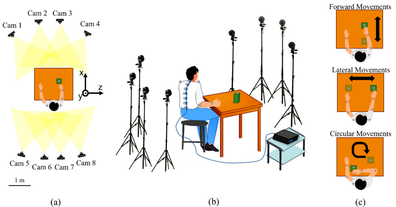
Figure 6. Experimental setup and protocol. (a) Upper view showing the positioning of the eight cameras and the reference axes. (b) The experimental set-up showing the subject's positioning, the MoCap system, the wearable system, and the spectrum interrogator. (c) Illustration of the three tasks performed during the protocol.
