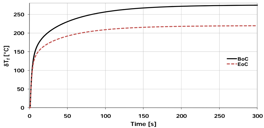
Fig. 11. Fuel average temperature variation following a step reactivity insertion of 50 pcm.
