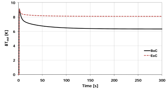
Fig. 16. Core outlet temperature variation following an enhancement by 10 K of core inlet temperature.
