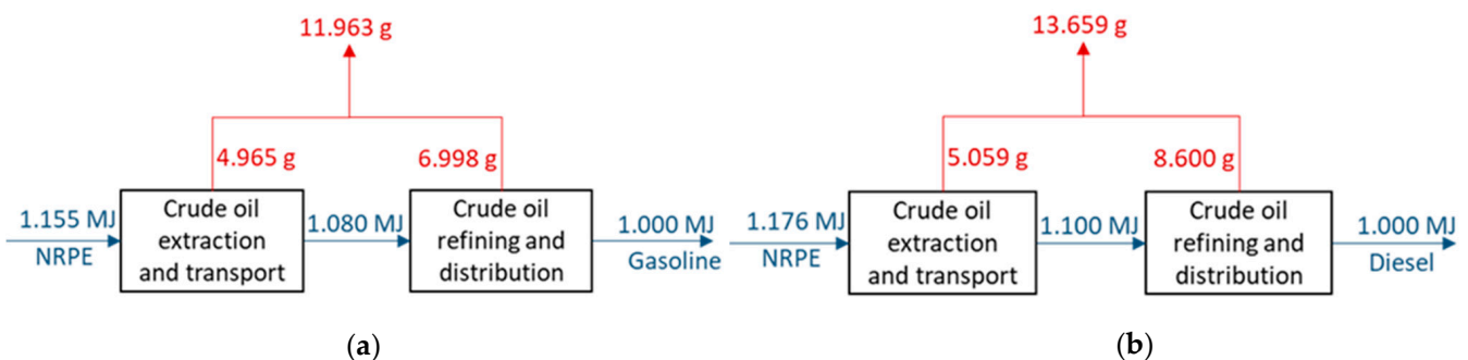
Figure 3. WTT analysis for gasoline (a) and diesel (b) [12].
