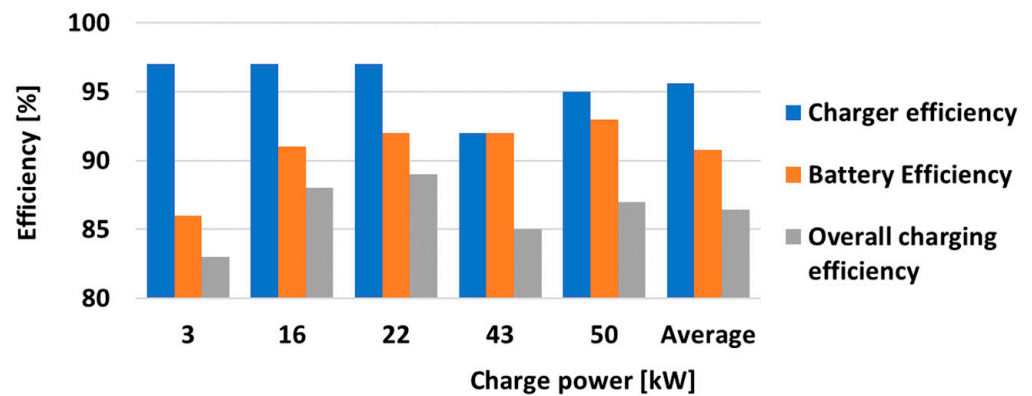
Figure 1. Charger efficiency, battery efficiency, and overall charging efficiency by the power of the charging system (with average values).
