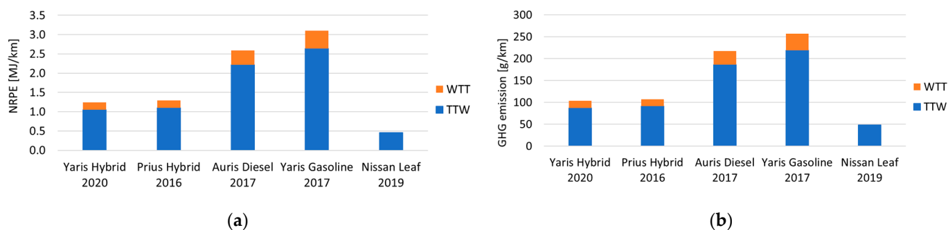
Figure 4. Specific NRPE (a) and specific GHG emission (b) of the vehicles analysed.
