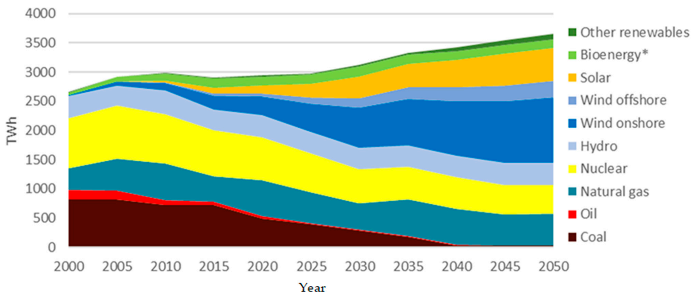
Figure 8. Gross electricity generation by year and power plants, the * represents renewable energy generated through biomass fuel burning.
