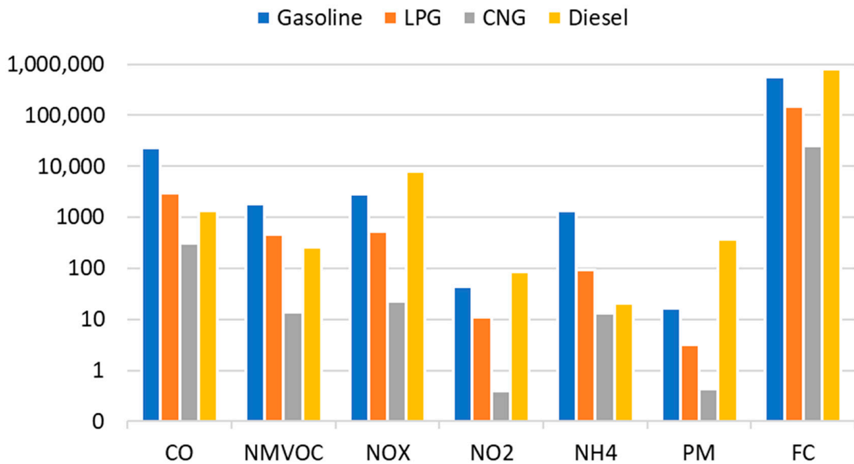
Figure 7. Emissions and FC divided by fuel type in 2021.
