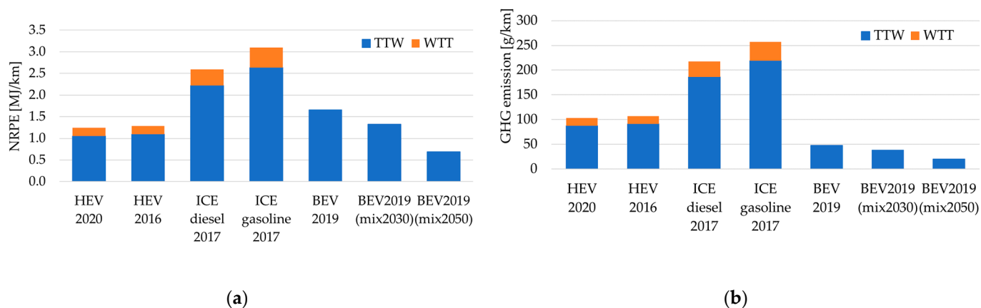
Figure 9. Specific non-renewable energy consumption (a) and specific GHG emission (b) for HEV, BEV (current mix), BEV (mix 2030), and BEV (mix 2050).
