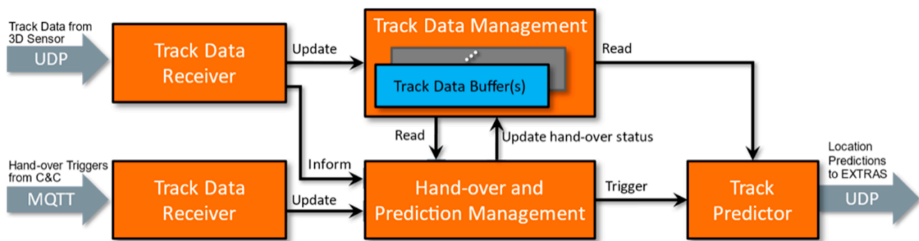
Figure 3. 3D Video software architecture.
