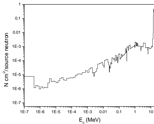
Figure 3 – 175 group VITAMIN-J unfolded neutron flux spectrum
