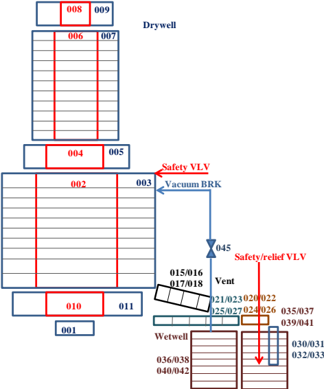
Figure 24: RELAP/SCDAPSIM TH nodalization of the MARK I containment
