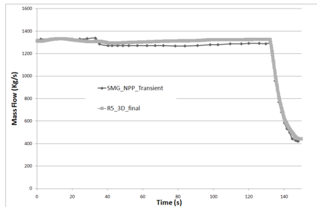
Figure 26: On-transient qualification: Recirculation line mass flows (kg/s), line A (left), line B (right)
