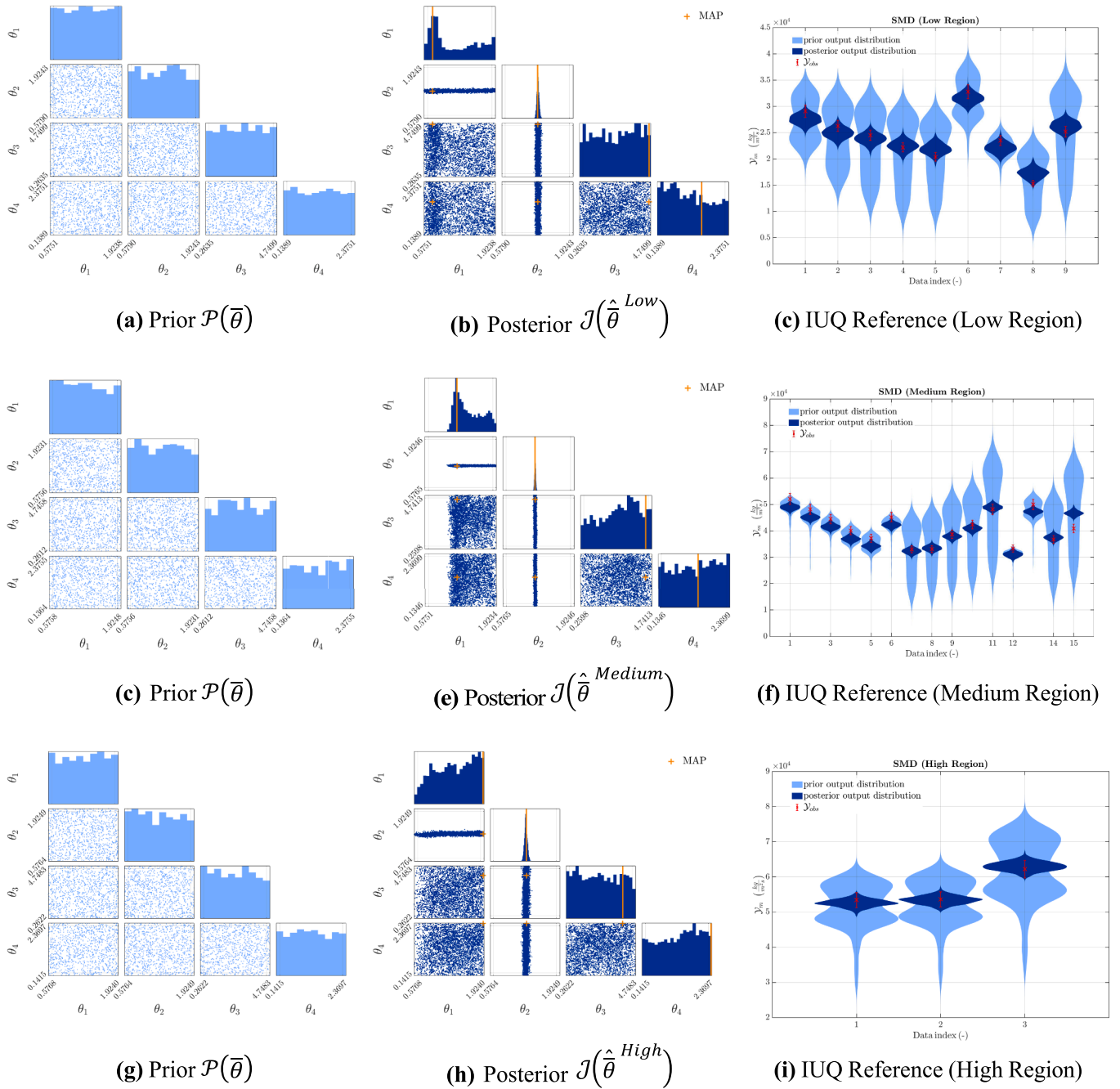
Fig. 10. Results of local IUQ analysis for SMD.
