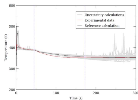
Figure 4. PC temperature (experimental data vs reference and uncertainty calculations results).
