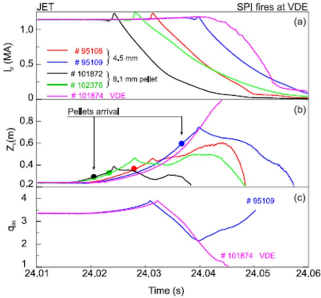
Figure 4. Suppression of VDE by SPI (a) plasma current, (b) current centroid vertical position, (c) q_{95} . Reproduced with permission from [41].
