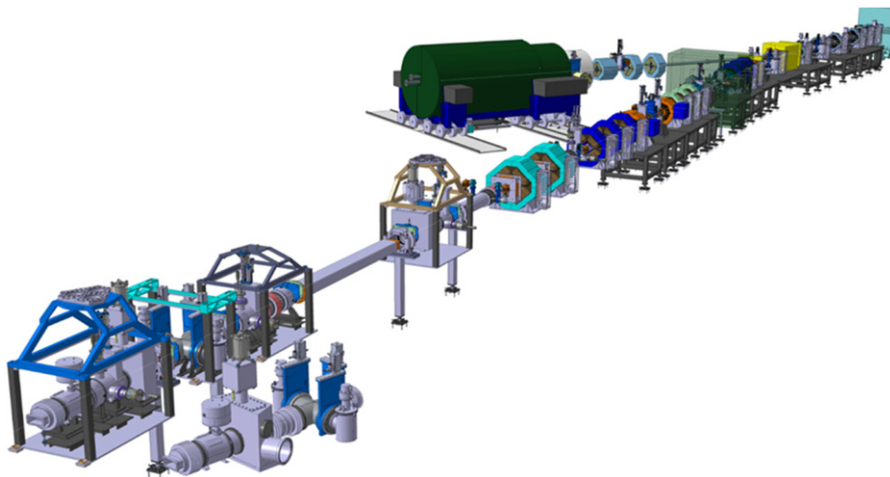
Figure 3. IFMIF-DONES HEFT. During the tuning phases of the accelerator at low duty cycle the beam is deviated to the beam dump (show in green) by a dipole magnet.
