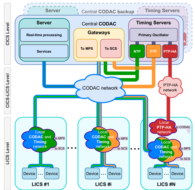
Fig. 3. Block diagram of a timing system that integrates into the existing network of the CODAC system of the I&C system at CICS, network and LICS levels. NTP is represented in green, PTP in orange and PTP-HA in red.
