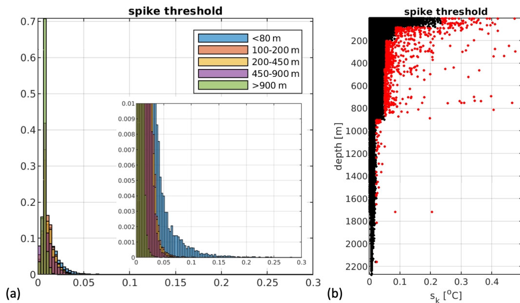
Figure 4. (a) Distribution in terms of probability of the spike threshold ( s_k ) in five layers, with a zoom probability of below 0.1 %. (b) Vertical distribution of the spike threshold, with values above the 0.999th quantile indicated in red.
