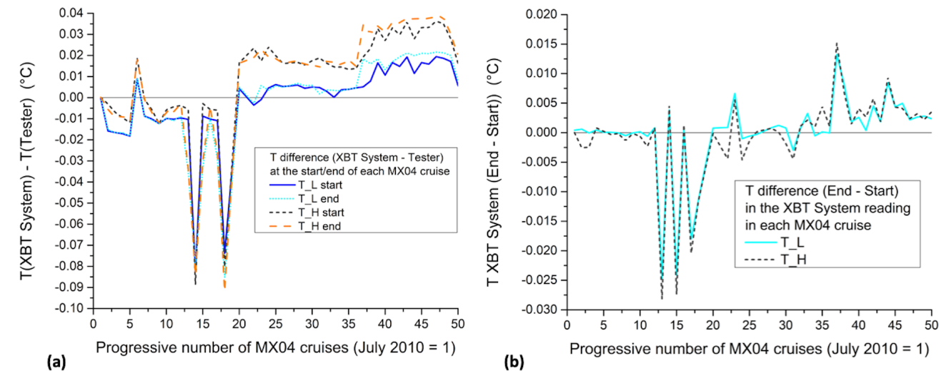
Figure 5. (a) Temperature difference (XBT system tester) obtained from the checks at the reference temperatures before starting and at the end of each MX04 cruise. (b) Difference between initial and final measurements, with the tester during the same cruise at the reference temperatures.
