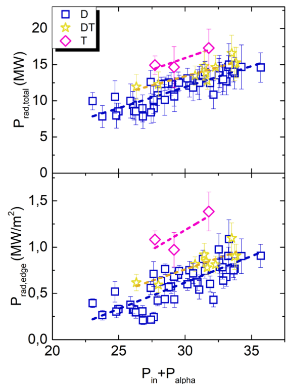
Fig. 1. The total radiated power P_{rad,total} (on the top) and the the edge line averaged radiation P_{rad,edge} (on the bottom) from a vertical bolometer channel as a function of the sum of input and the alpha particles powers for D, DT and T plasmas. Dashed lines indicate linear fit to particular data sets.
