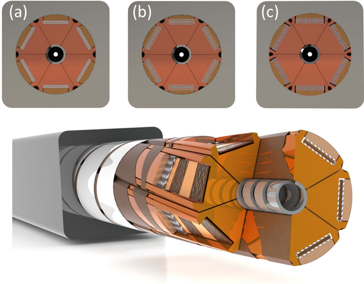
Figure 2. Schematic representation of the three cross-sections of the SECAS HTS Sector Shaped high-current Conductor considered in this work. Each sector contains: (a) one BRAST made of ten 12 mm-wide tapes; (b) two BRASTs, each made of five 12 mm-wide tapes; and (c) six BRASTs, each made of five 4 mm wide tapes. Bottom: perspective representation of the assembled SECAS conductor with BRASTs, sector-shaped core, fillers, outer steel wrap, and central spiral.
