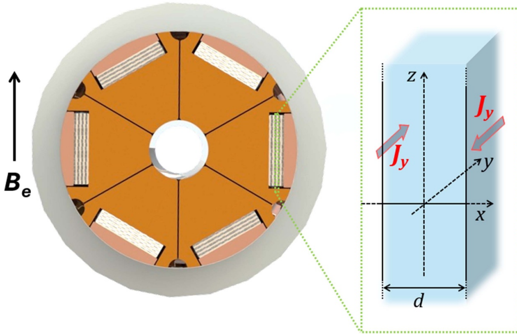
Figure 5. Schematic representation of the 1D Bean's slab model and the coordinate system used for modeling a superconducting stack subjected to an external field parallel to the flat surface of the tapes. Each tape is represented by an infinite slab of thickness \delta oriented in the y, z -plane with an externally applied magnetic field B_e directed along z direction. The induced shielding current density J_y flowing in the y direction inside the front and back faces is shown.
