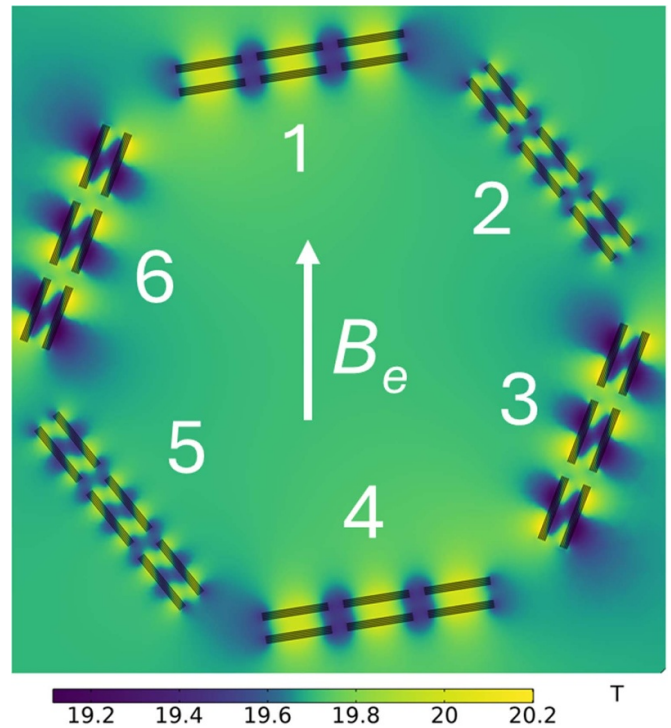
Figure 12. Magnetic field distribution in the Option-C cable, calculated at T = 4.2 K at time instant t/T = 0.29 .
