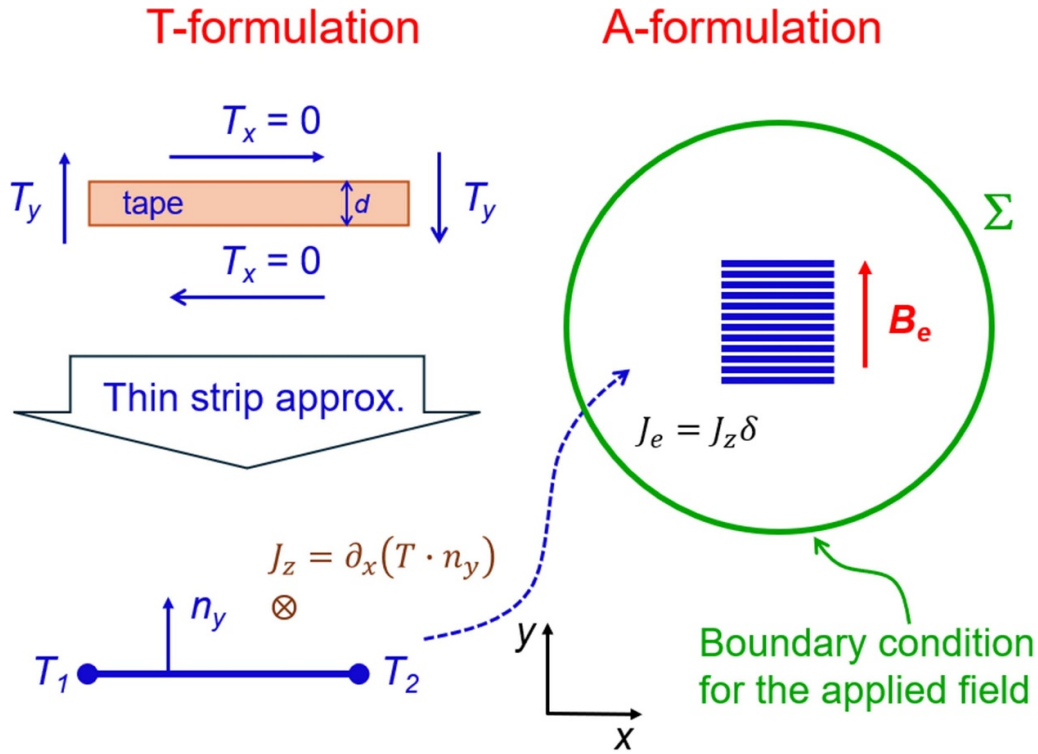
Figure 4. Schematic representation of the 2D T-A model and the coordinate system used for modeling a superconducting stack subjected to an external field oriented perpendicularly to the flat surface of the tapes. The current vector potential \mathbf{T} is evaluated only in the superconducting strips, whereas the vector potential \mathbf{A} is computed everywhere. The screening currents are enforced by boundary conditions at the edges T_1 and T_2 of the tape ( T_1 = T_2 = 0 ).
