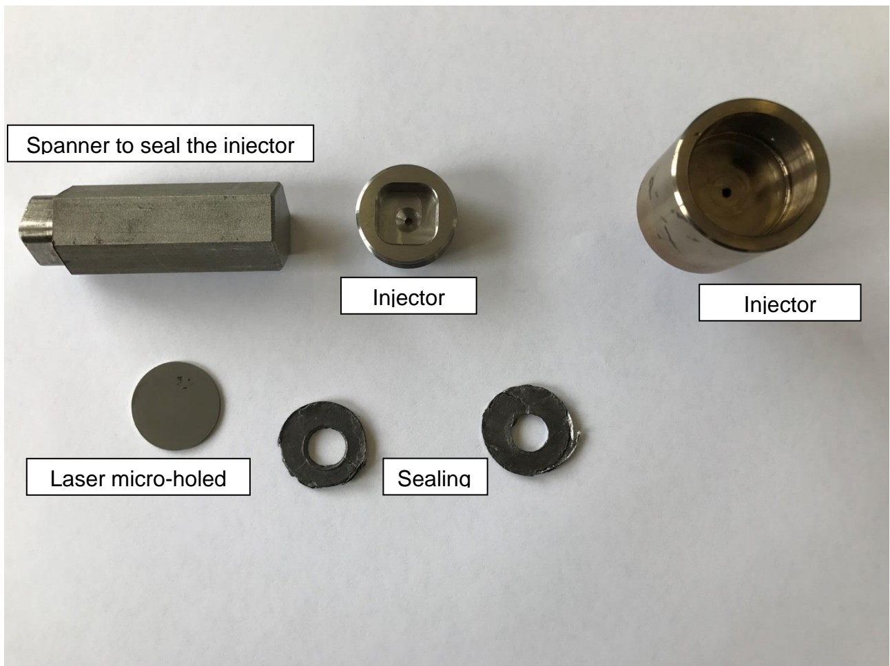
Fig. 13 – Injector system device.
