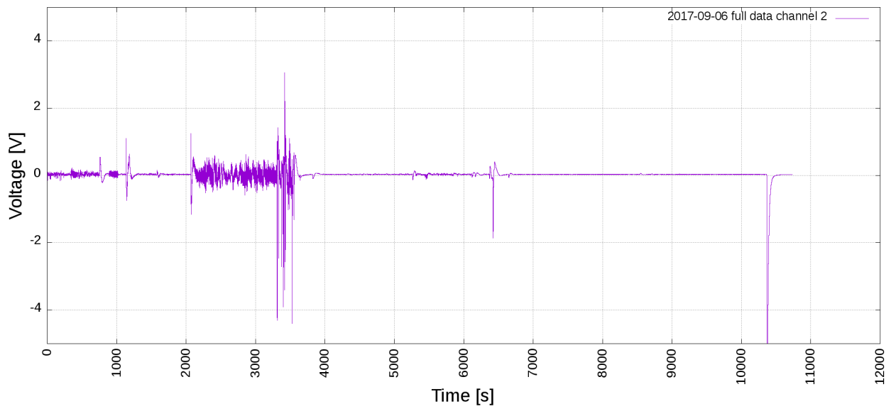
Fig. 42 – Test C1.1_60, raw data channel 2 [time domain].
