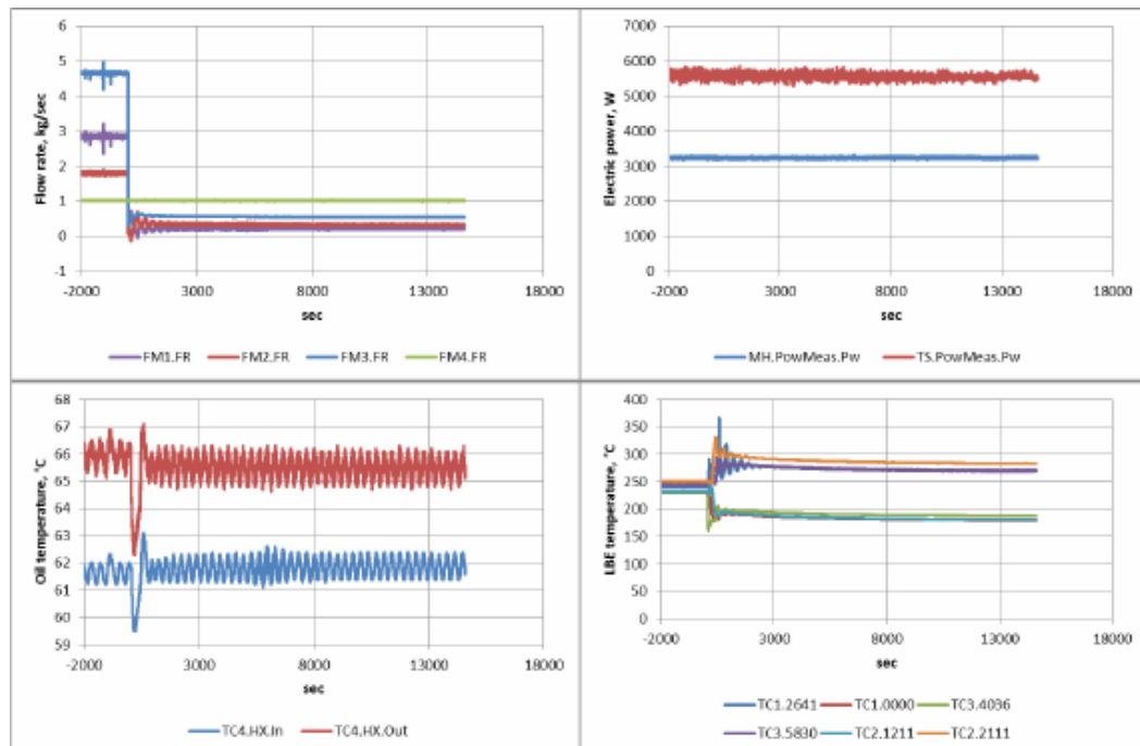
Fig. 4.2 - Experimental data for test series TG03S301.
