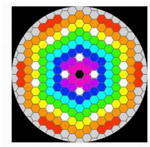
Fig. 5.6 – Identification of the concentric regions at the same temperature (generated by FRENETIC) adopted for the Serpent run.
