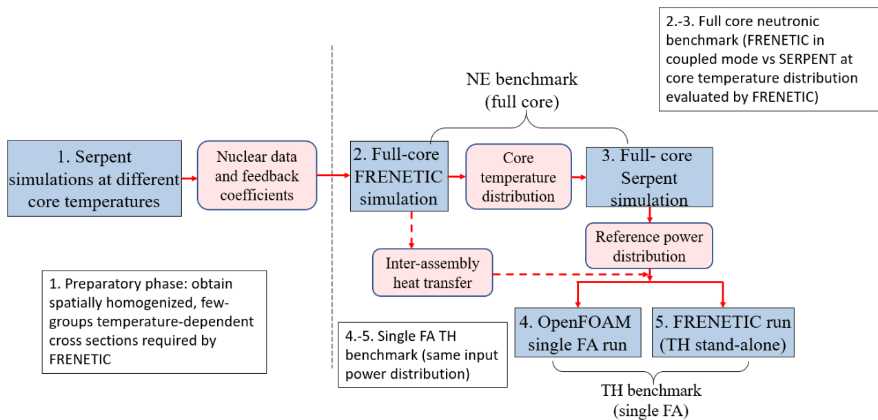
Fig. 5.5 – Coupling scheme and definition of simulation phases.
