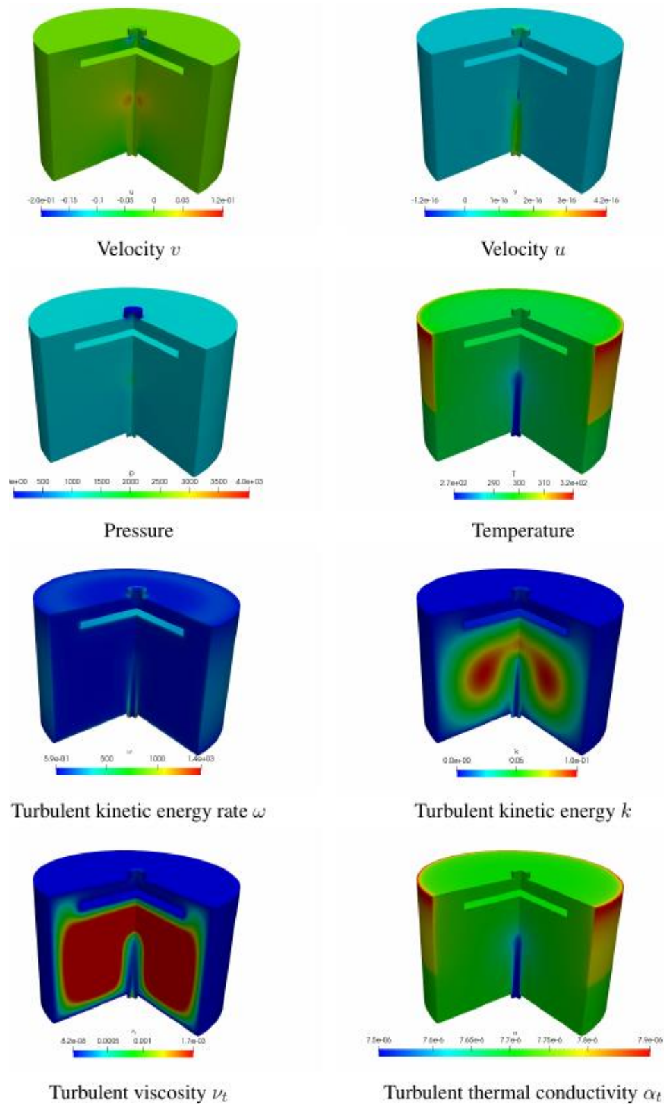
Fig. 4.13 - Initial steady state for turbulent variable for CFD OpenFoam code with the turbulent flow model \kappa\text{-}\omega .
