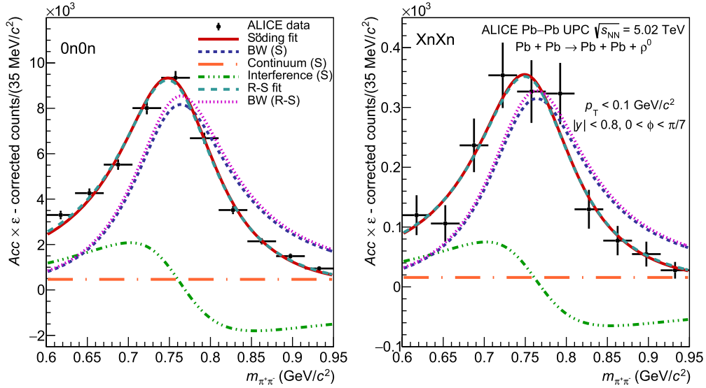
Fig. 1. Invariant-mass distribution of pion pairs, with superimposed Soding (solid line) and Ross-Stodolsky (dotted line) fits, for the range 0 < \phi < \pi/7 in the On0n (left) and XnXn (right) neutron classes. The different components of the pion-pair production amplitude in the Soding model are shown: the Breit-Wigner shape that describes the \rho^0 (finer dotted line), the continuum process (dash-dotted line), and the interference between the \rho^0 and the continuum (dash-dot-dot-dot line). The Breit-Wigner extracted from the Ross-Stodolsky model (finest dotted line) is also shown. In this example, the background contribution from misidentified muons is fixed to zero in the fit.
