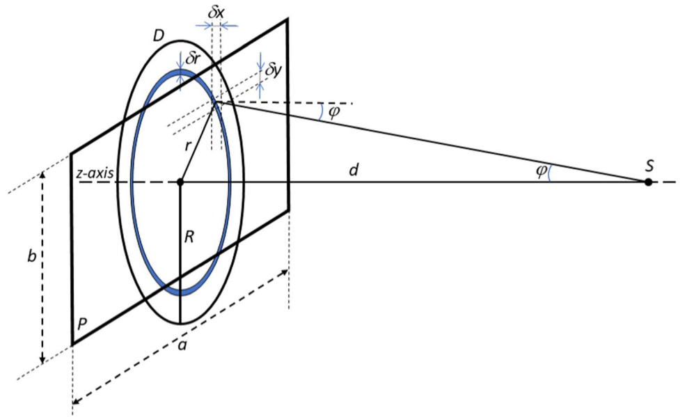
Figure A1. Schematics showing the geometry for deriving equations (A2) and (A5). A luminous plane ( P ) of sides a and b is separated by a distance d from the light sensor ( S ). An infinitesimal plane element of area \delta x \delta y illuminates the sensor along a direction forming an angle \varphi with the disc surface normal. The luminous plane is approximated by a concentric luminous disc ( D ) of radius R = [(a \times b)/\pi]^{1/2} . An infinitesimal concentric ring of radius r and thickness \delta r illuminates the sensor along a direction forming an angle \varphi with the disc surface normal.
