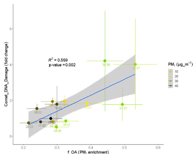
Fig. 6. Exposure-response curves of A) Comet assay ( n = 14 ) results vs the enrichment of PM 1 in organic aerosol (OA). The Comet-OA curve, statistically significant, and with a high R^2 = 0.559 , underline the relevance of the chemistry determining atmospheric aerosol toxicological properties rather than the airborne mass, number, or surface area exposure doses. Noteworthy, higher DNA damaging effects were related to low PM 1 airborne concentrations.
