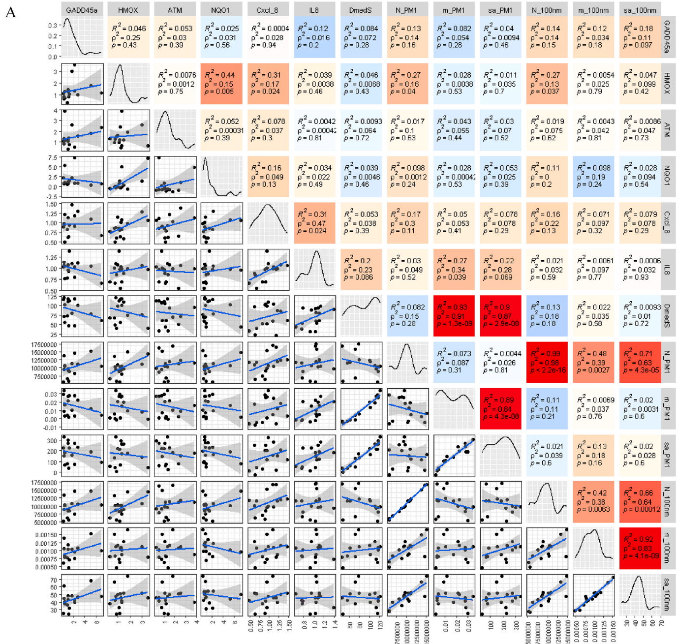
Fig. 2. Pearson (R 2 ) and Spearman (ρ 2 ) correlation matrix of modulated genes (A) and DNA damage endpoints (B) and exposure doses expressed as deposited number, deposited mass, or deposited surface area of the total PM 1 and UFP particles (n = 16). Reddish background stands for a positive association while bluish background for negative ones. The significance of the association is reported as p value in each box. The diagonal plots report the data interpolated distribution of the data.
