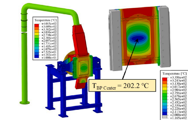
Fig. 15. FEM analysis of the thermal field in the DRP TA prototype at the end of pre-heating.
