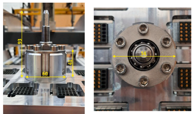
Fig. 12. EC bridge central screw: (left) lateral view, (right) top view.
