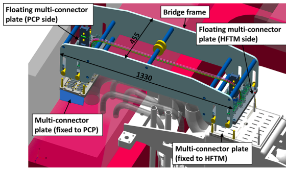
Fig. 7. 3D model of the HFTM electric connectors bridge. Dimensions are in mm.
