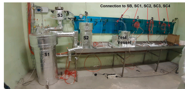
Fig. 4. Overall view of ANGEL plant, with one of the test vessel connected (SB). Other vessels can be similarly connected to the indicated, adjacent positions.
