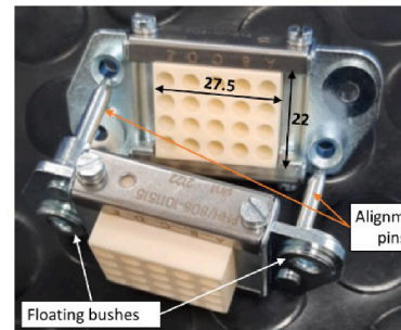
Fig. 11. 3D model (top) and as-built mock-up (bottom) of the single 20-pin alumina connector. Dimensions are in mm.
