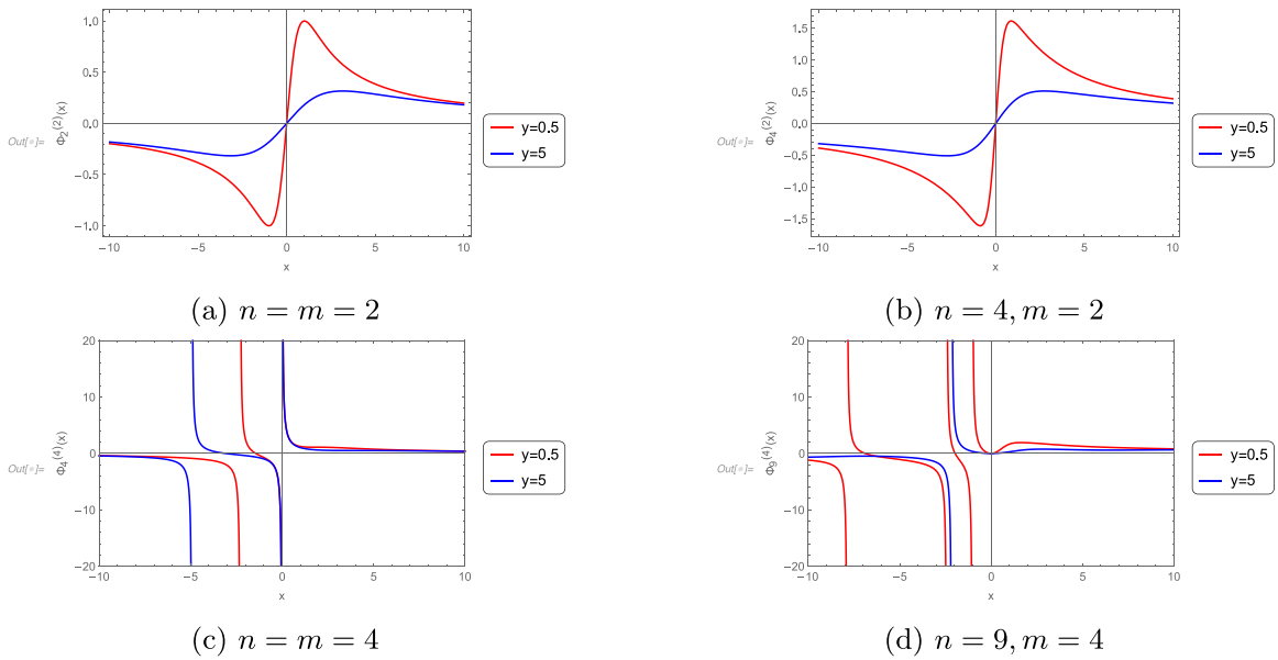
Fig. 1. Comparison of \Phi_n^{(m)}(x, y) vs. x for fixed y values and different n and m values.
