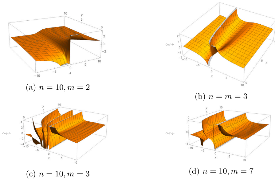
Fig. 2. Eq. (4.8) for different n and m values.
