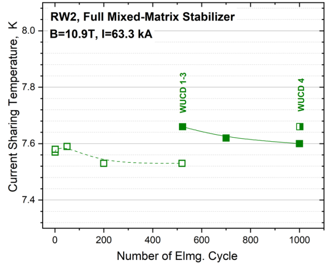
Fig. 2. The T_{cs} performance of RW2 as a function of em and thermal cycles in 2018 (no bending). The empty symbols are from the first campaign, followed by three WUCD, the second campaign (full symbols) and a final WUCD.
