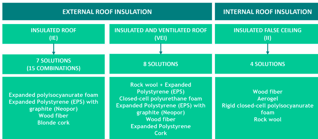
Figure 8. Prefabricated insulation solutions available on the market.
