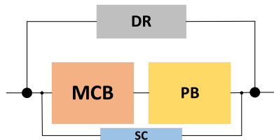
Fig. 2. Block diagram of one FDU, composed by the MCB, a snubber circuit (SC), the PB and a DR.
