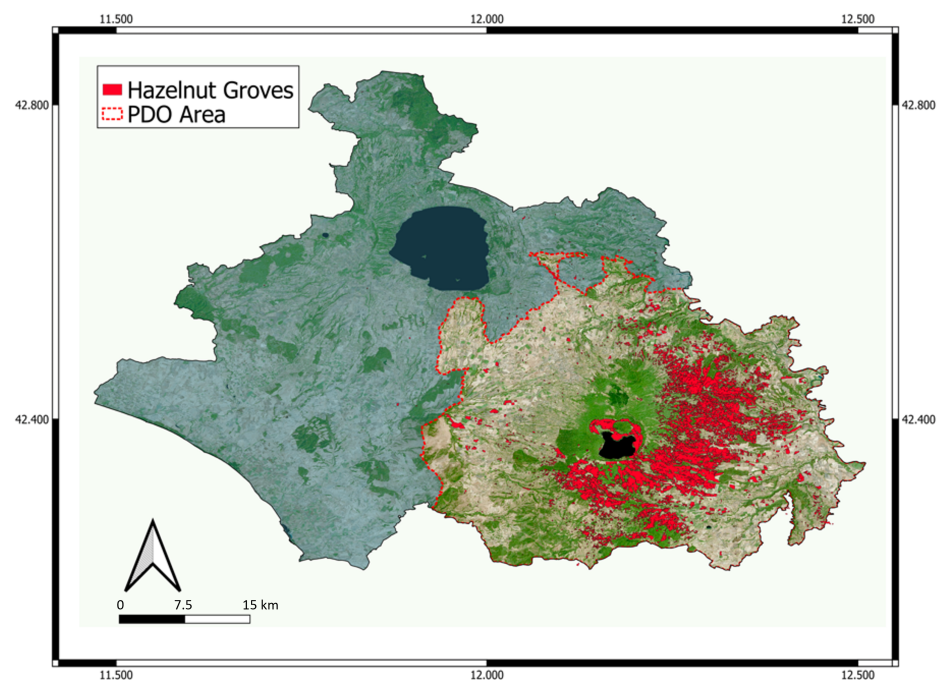
Figure 11. Map of the area occupied by HZ within the AOI.
