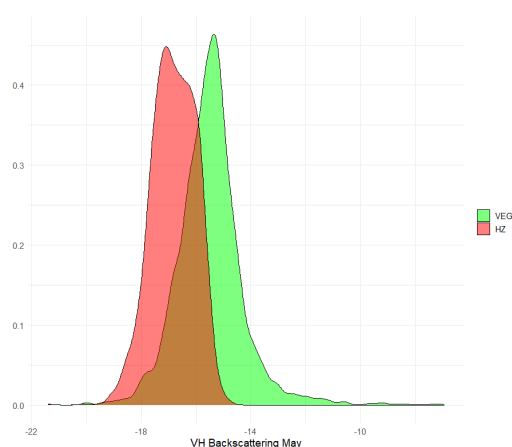
Figure 20. Density plot for VHV backscattering in May.
