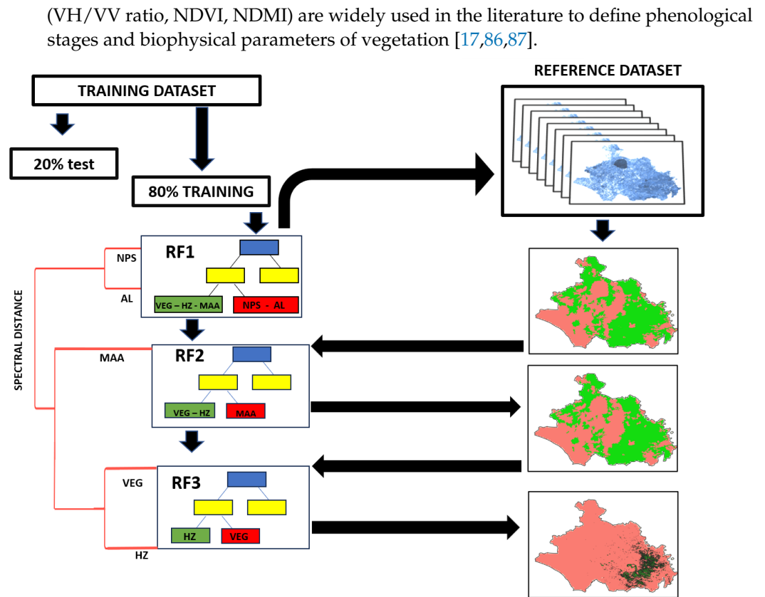
Figure 6. Workflow for Hierarchical Random Forest training via Euclidean distance analysis of spectral signatures.
