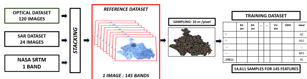
Figure 5. Creation of the Reference Dataset through Stacking and Training Dataset at 10 m/pixel Sampling.
