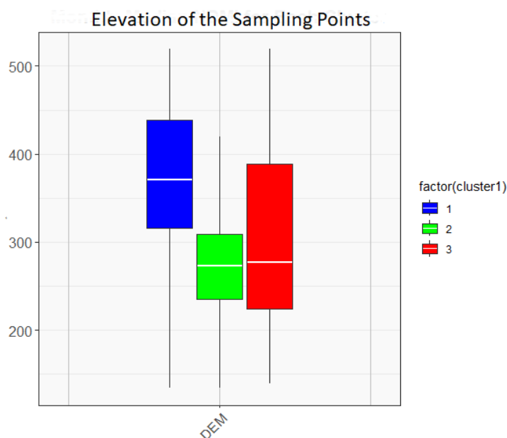
Figure 18. Sampling points elevation values in different clusters (meters above sea level).
