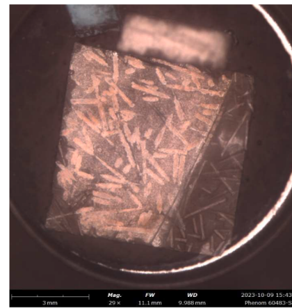
a) Optical image of a Wf/W specimen with dimensions 7x7 mm.
