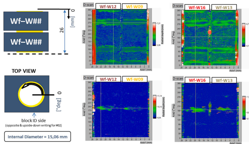
Fig. 11. UT d-scans of Wf/W-Cu blocks back-wall echoes.
