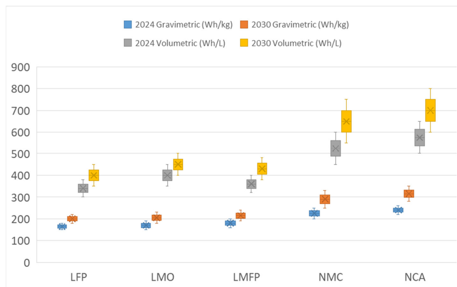
Figure 4. Evolutionary roadmap of lithium-based chemistries 2023–2030.
