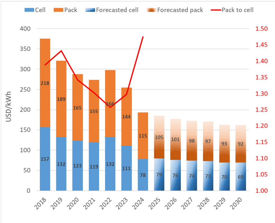
Figure 3. Pack and cell price trend from 2018 to 2024 [8]. The pack-to-cell price ratio is represented by the red line. Forecasted prices are reported for the 2025–2030 period.
