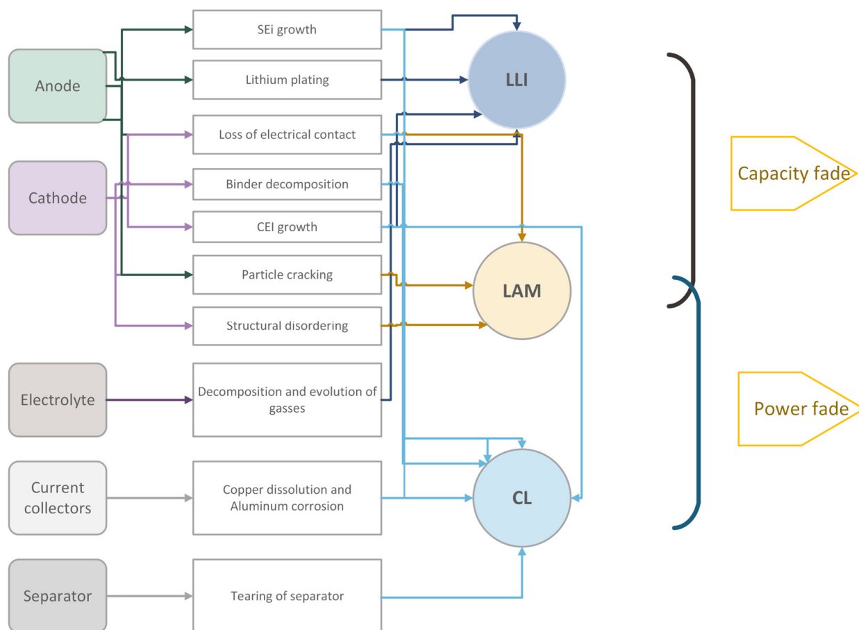
Figure 5. Schematic of degradation mechanisms and modes for different battery components.
