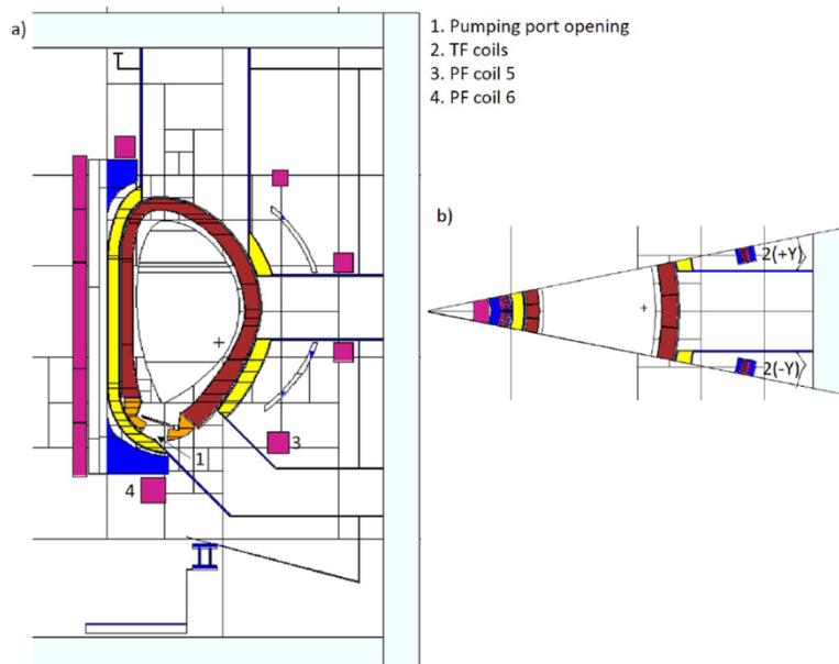
Fig. 2. MCNP geometry of the SN model for (a) vertical ( Y=0 ) and (b) horizontal ( Z=0 ) slice.
