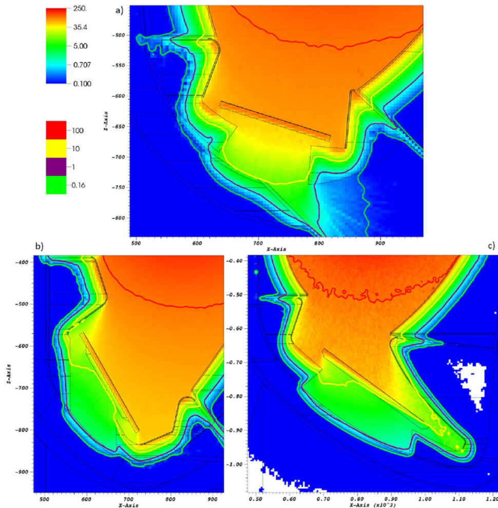
Fig. 8. He production (appm/FPY) in Eurofer for the (a) SN (b) XD and (c) SX configurations at Y=0 .
