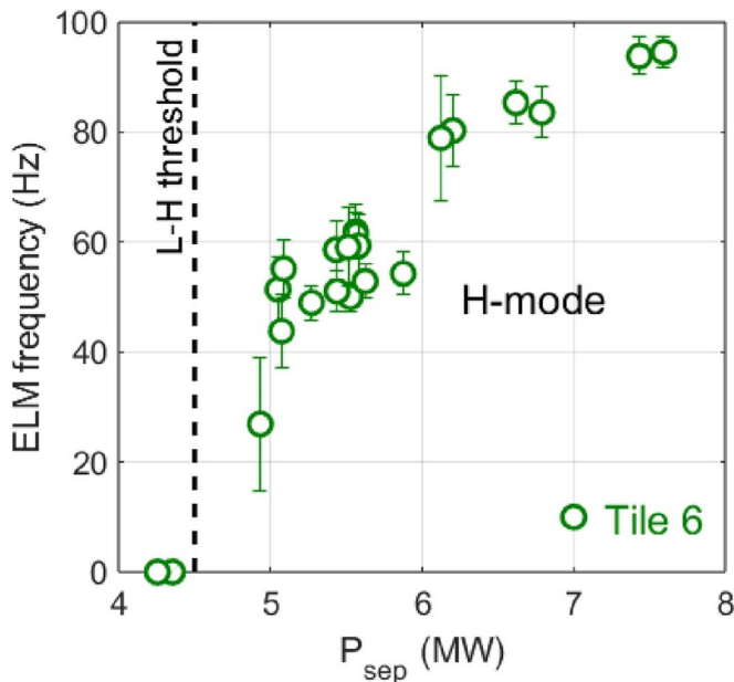
Figure 10. ELM frequency as function of the power flowing through the separatrix ( P_{\text{sep}} = P_{\text{IN}} - P_{\text{rad,bulk}} ) for operation on the Tile 6 divertor plate. The L–H power threshold is approximately 4.5 MW in all the pulses used.
